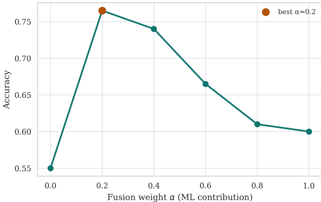
accuracy vs alpha
