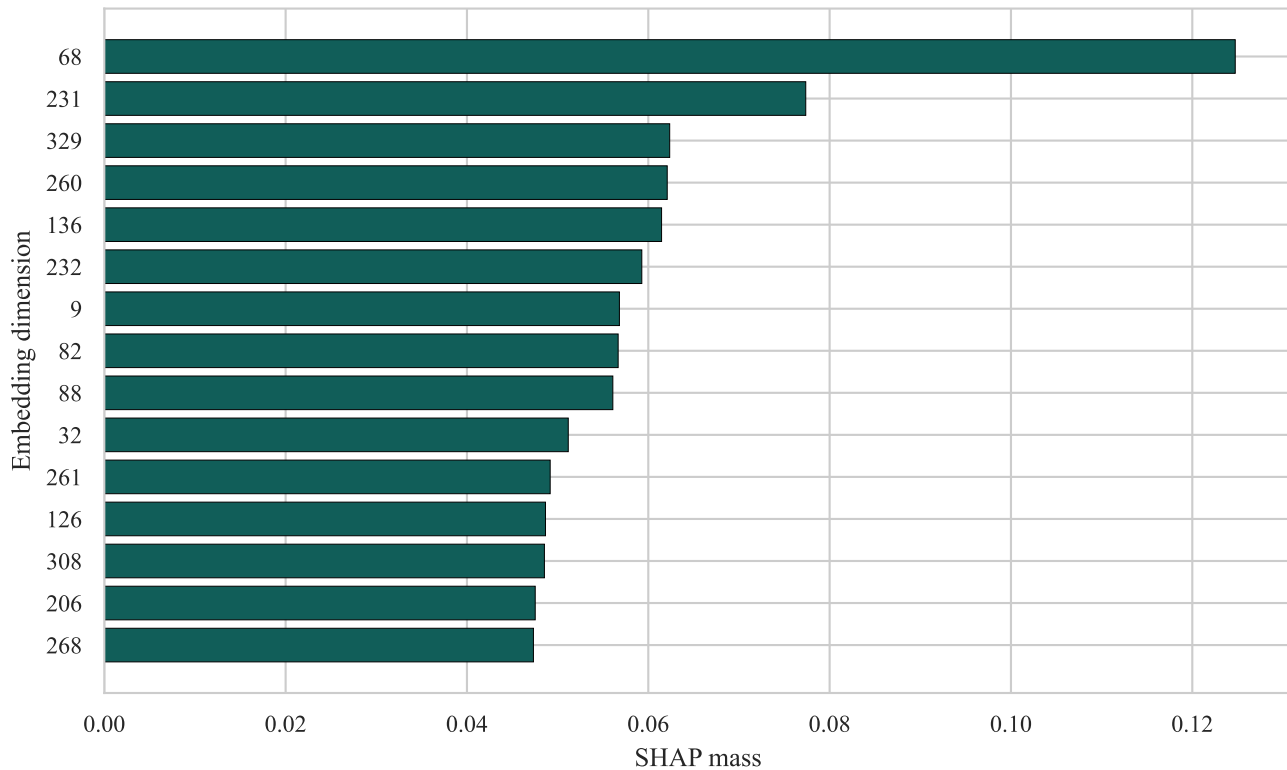
Global mean |\text{SHAP}| importance
