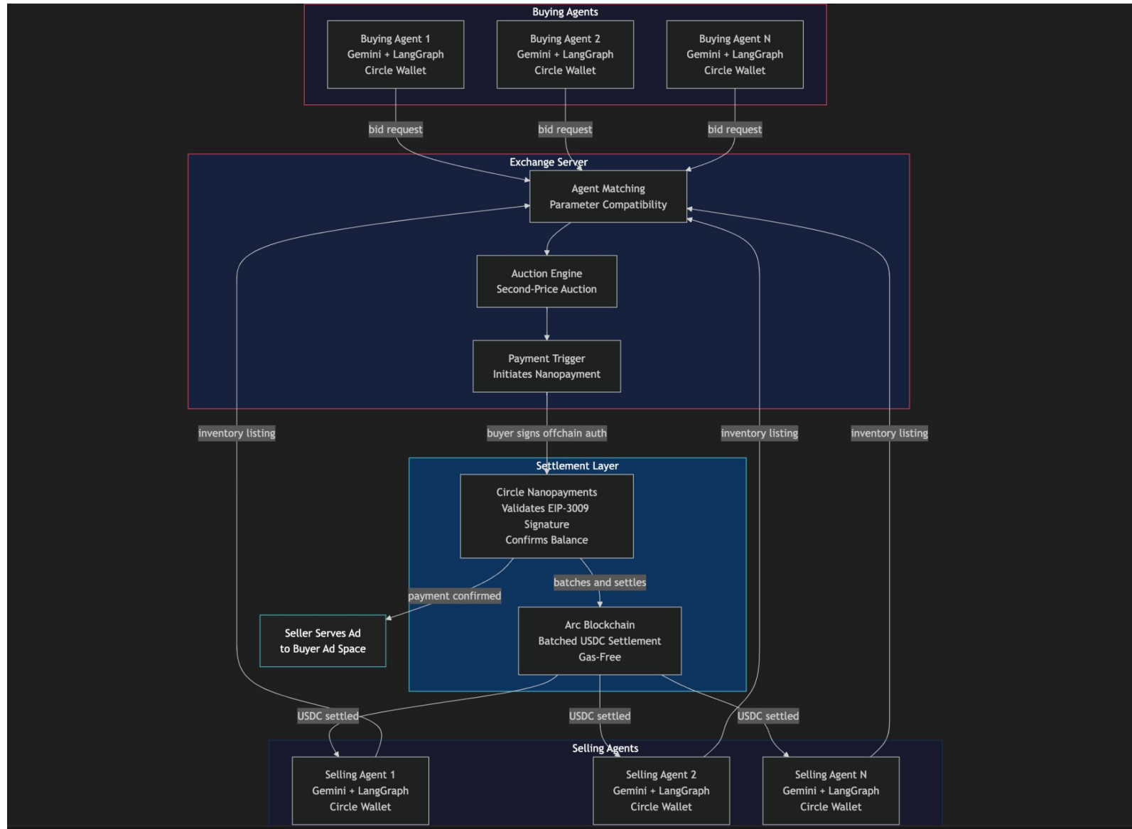
VDX System Architecture V1
