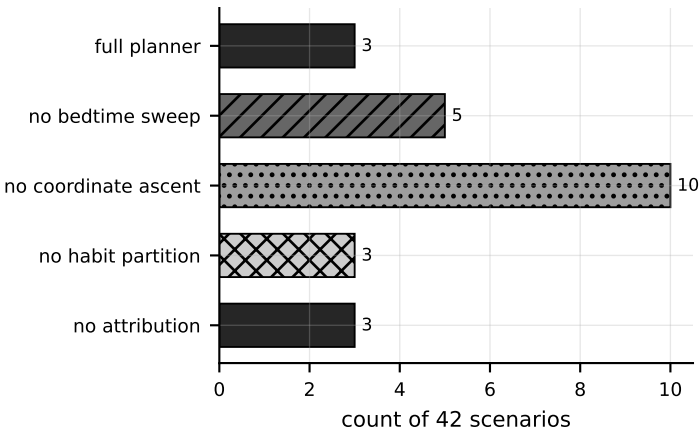
false refusals (conservative)
