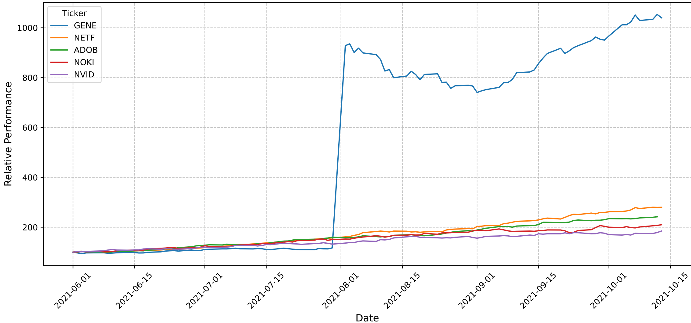
Relative Price History (Indexed to 100 on Start Date)
