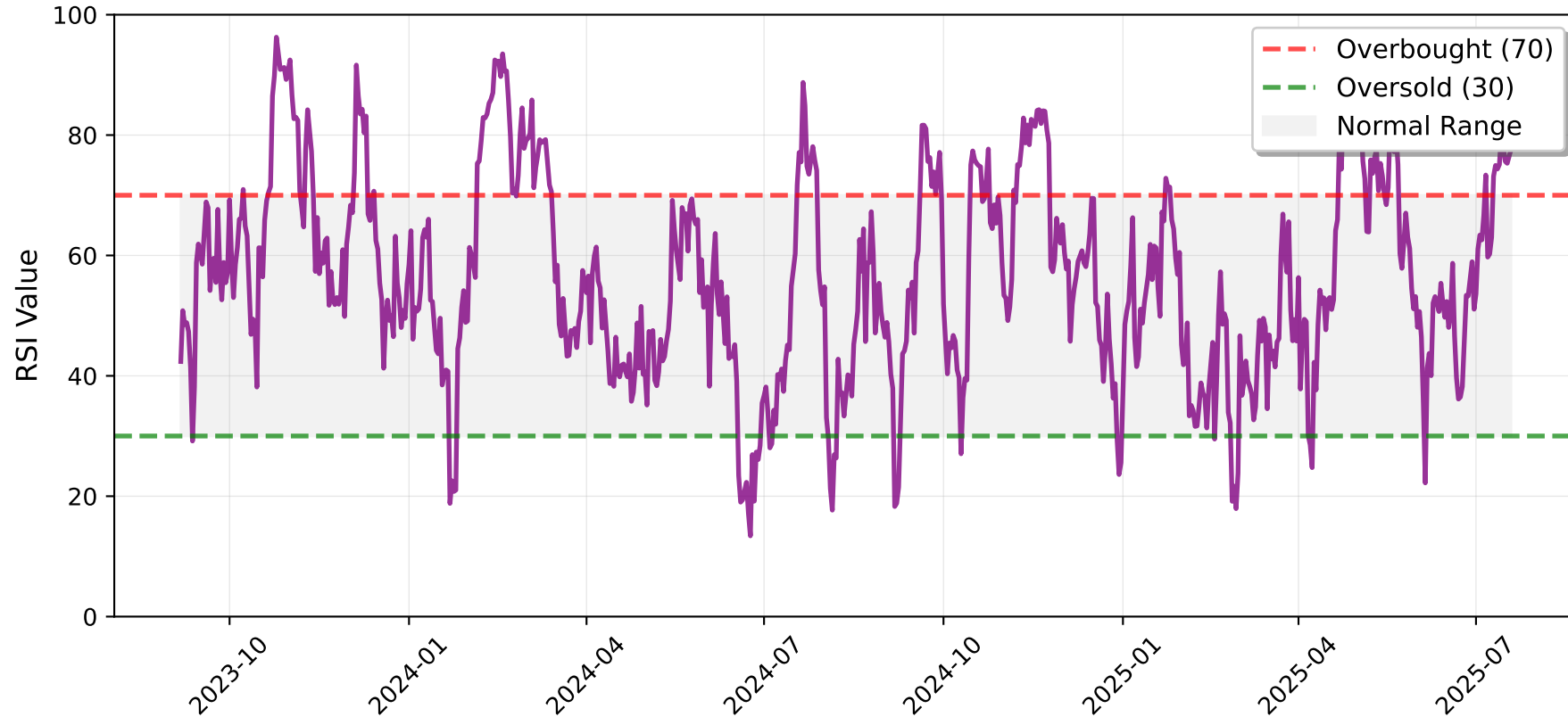
RSI Technical Indicator
