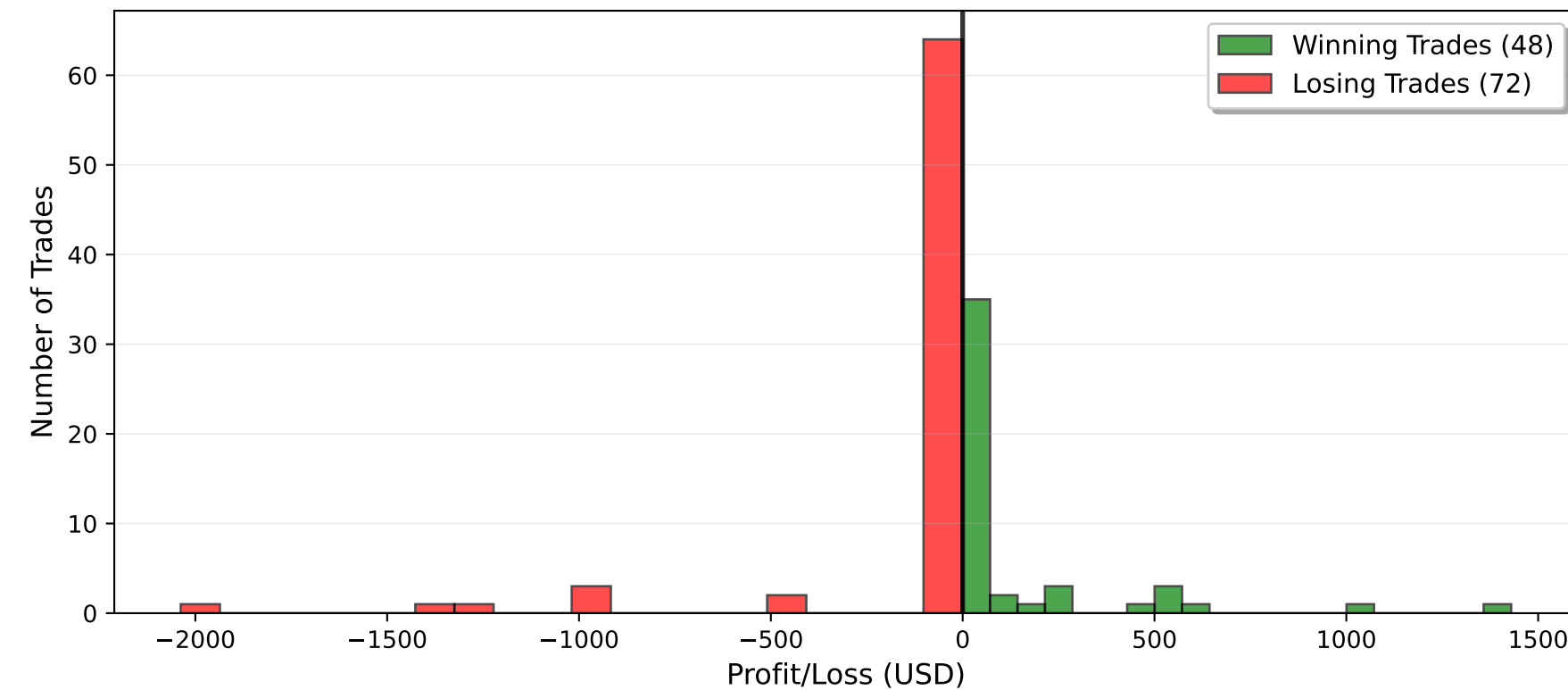
Trade P&L Distribution
