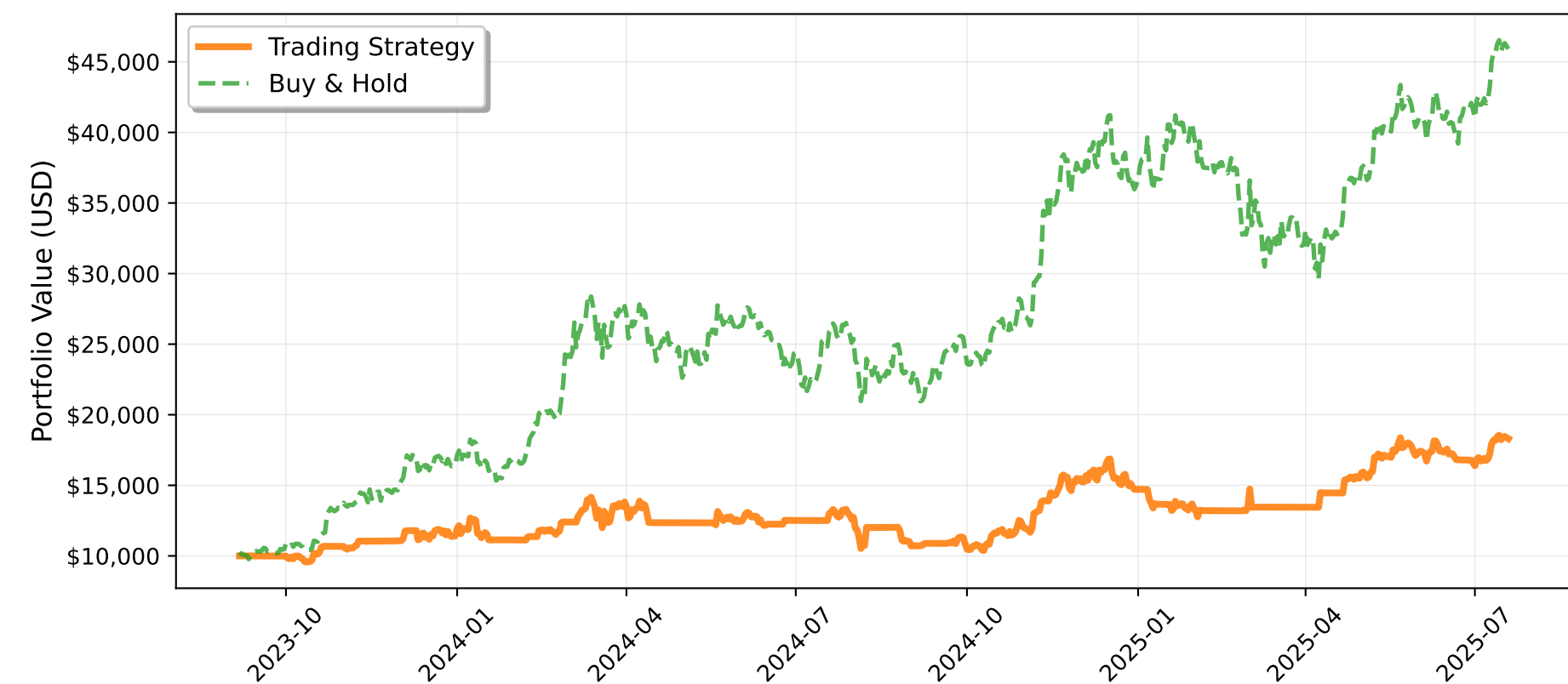
Portfolio Performance Comparison
