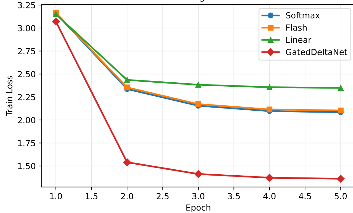
Training Loss
