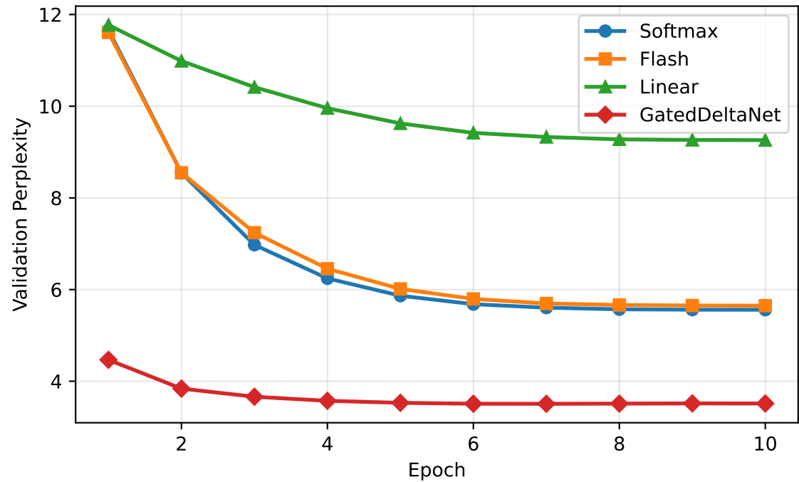
Validation Perplexity
