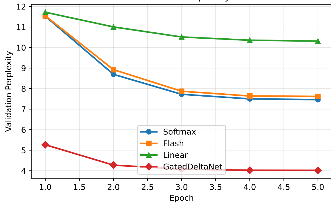
Validation Perplexity
