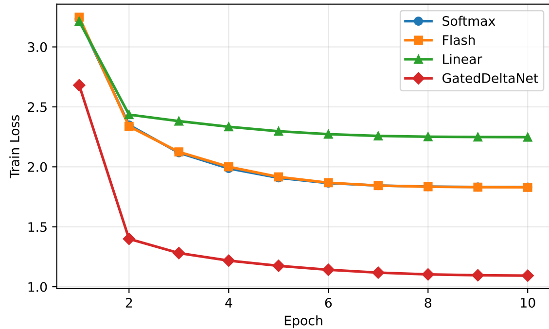
Training Loss
