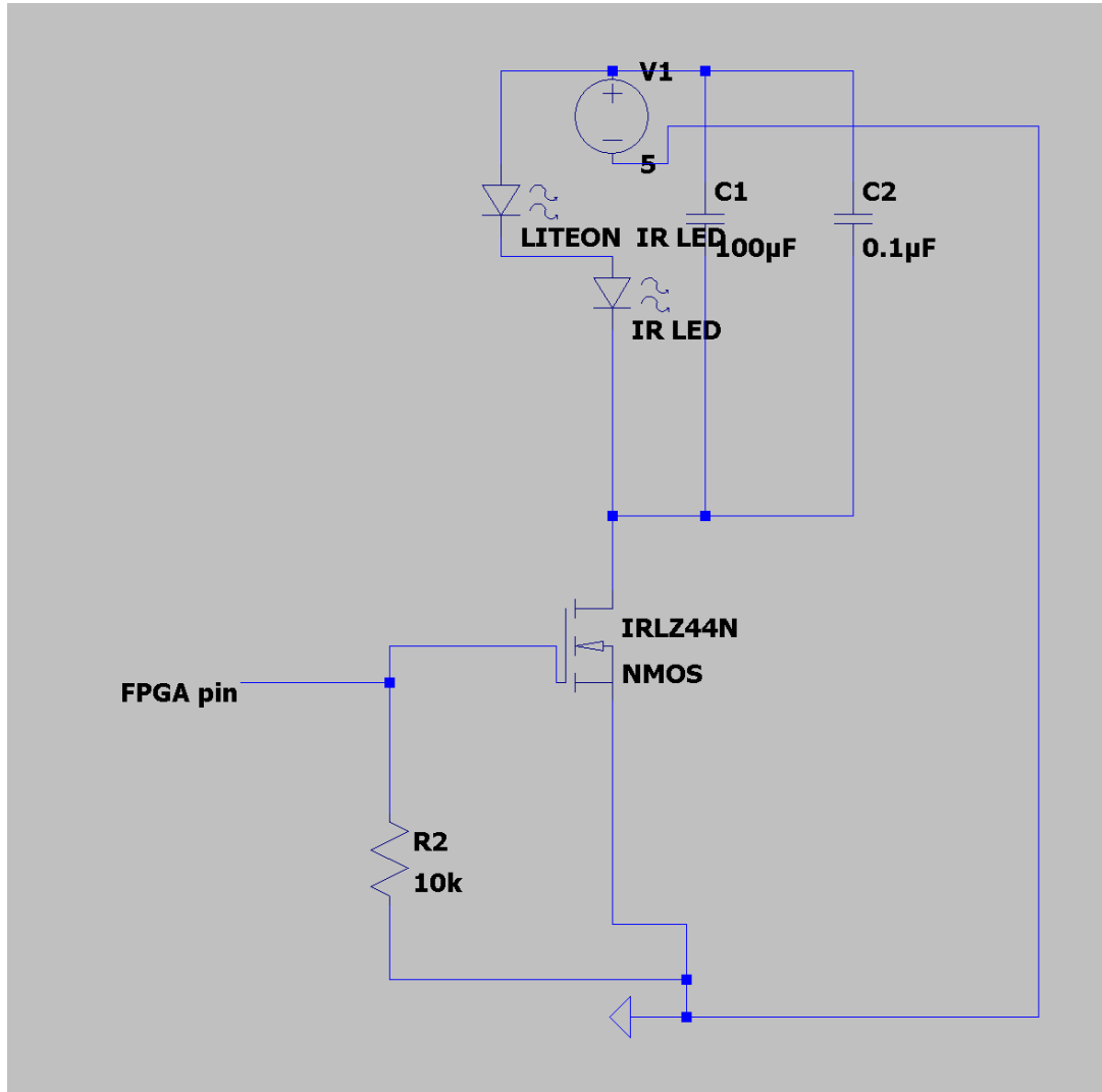
Figure 6: Complete 1A IR LED driver circuit with MOSFET switching.
