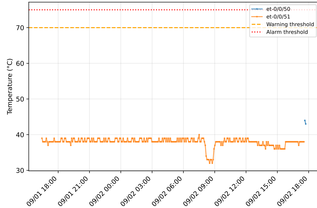
Module Temperature
