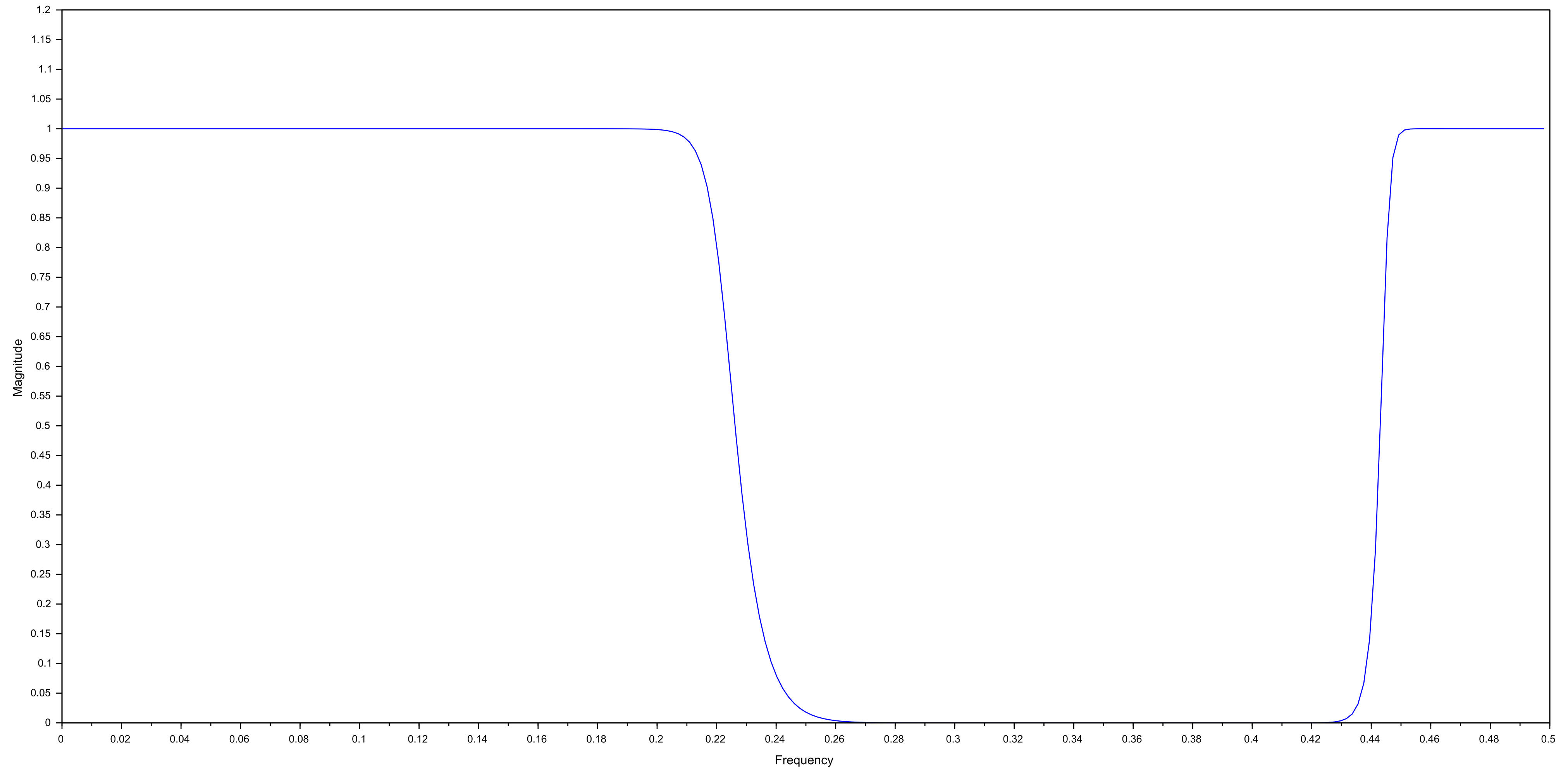
Butterworth IIR Band stop Filter
