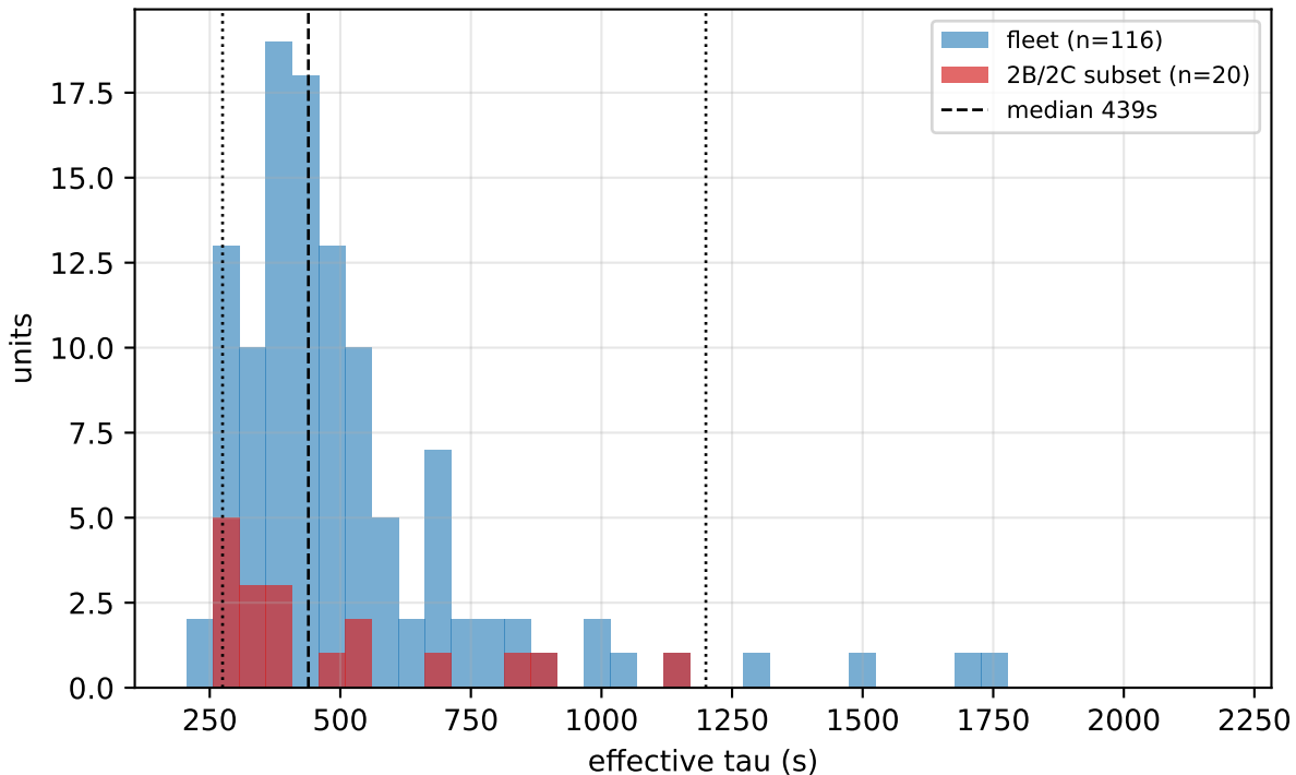
Figure 4. Fleet-scale distribution of effective tau (116 units)
