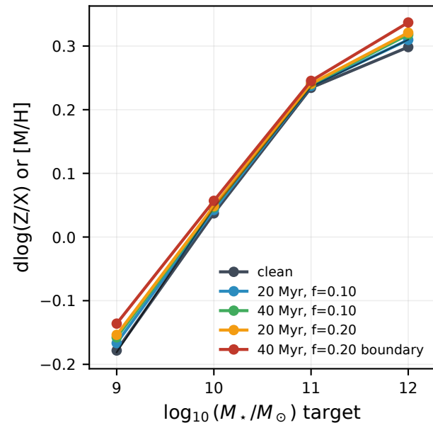
Mass-metallicity
