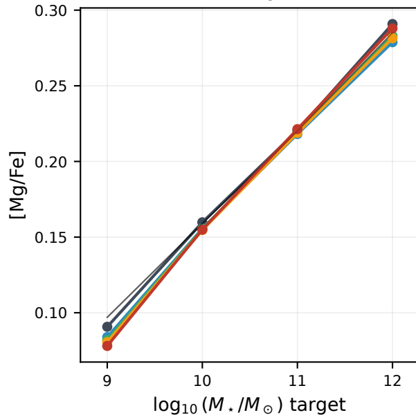
Mass-[Mg/Fe]
