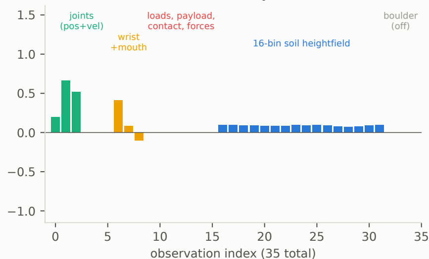
(b) What the POLICY sees: body + coarse soil (35-dim)
