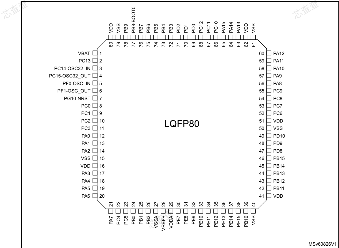
Figure 8. STM32G474xB/xC/xE LQFP80 pinout
