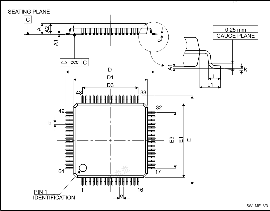
Figure 62. LQFP64 - Outline
