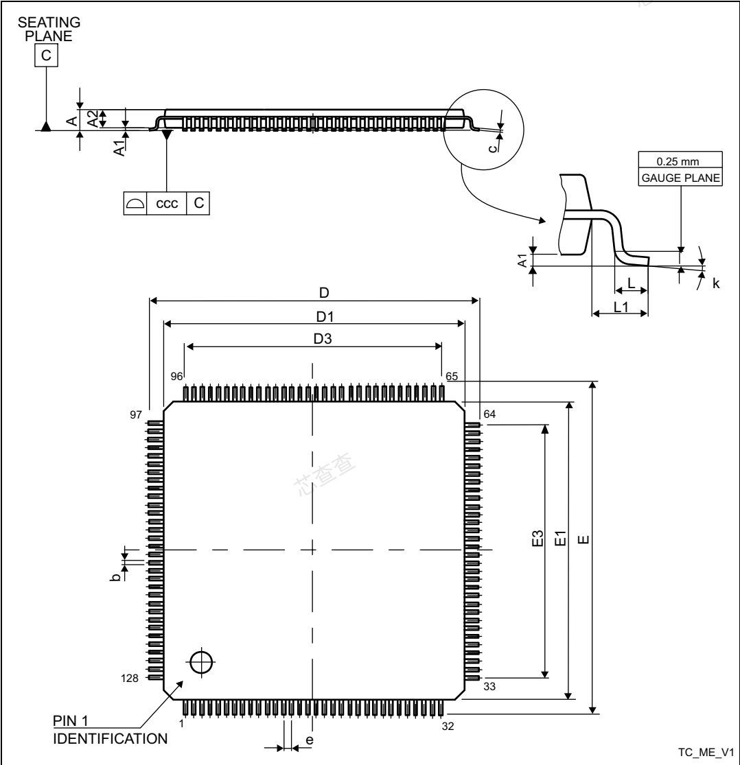
Figure 74. LQFP128 - Outline
