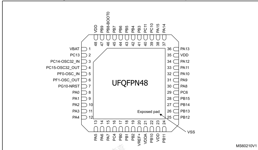
Figure 5. STM32G474xB/xC/xE UFQFPN48 pinout
