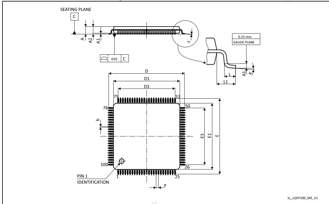
Figure 71. LQFP100 - Outline
