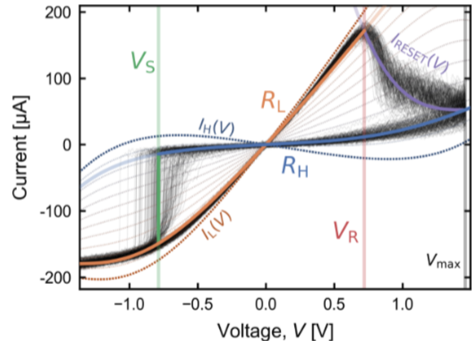
Figure: I–V characteristic curve of a memristor [Hennen + 24]
