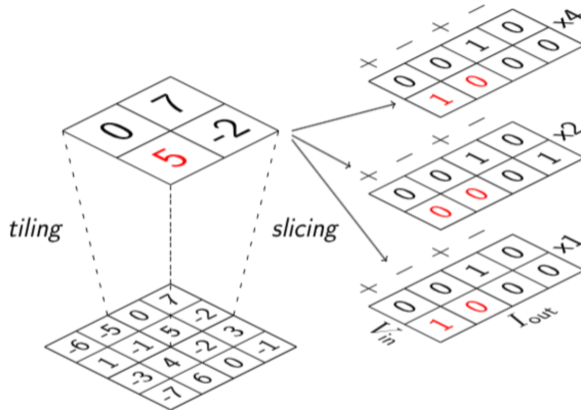
Figure: Mapping a weight matrix on memristor arrays [Rossenbach + 25]
