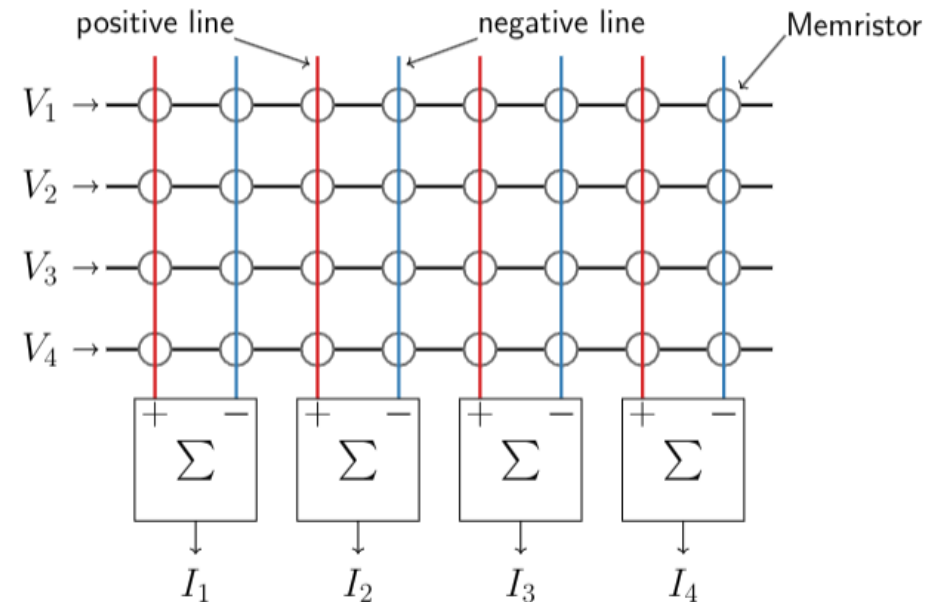
Figure: Paired memristor array structure [Aguirre + 24]
