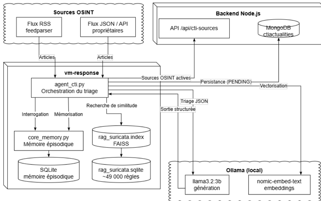
FIGURE 4.1 – Architecture du sprint 4
