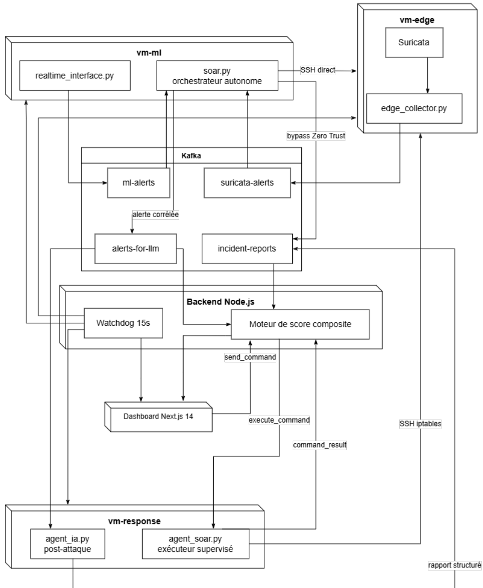
FIGURE 4.18 – Architecture du sprint 6
