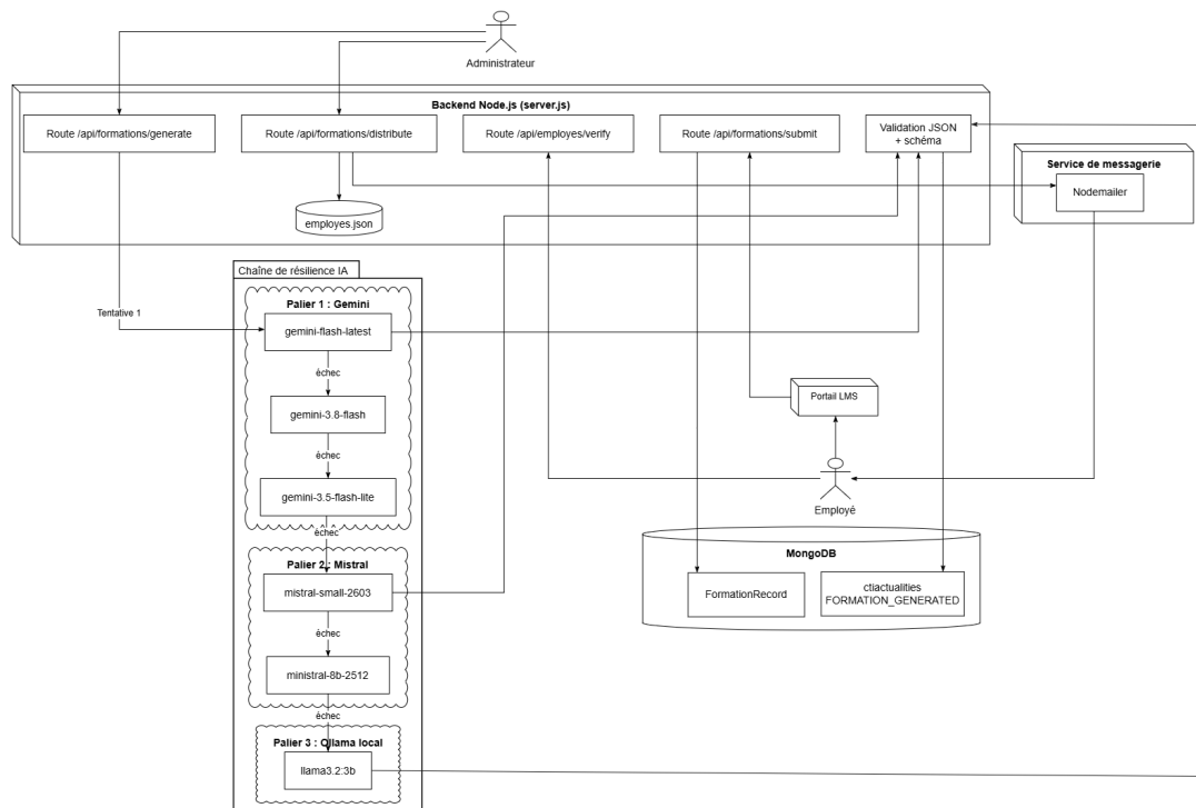
FIGURE 4.10 – Architecture du sprint 5
