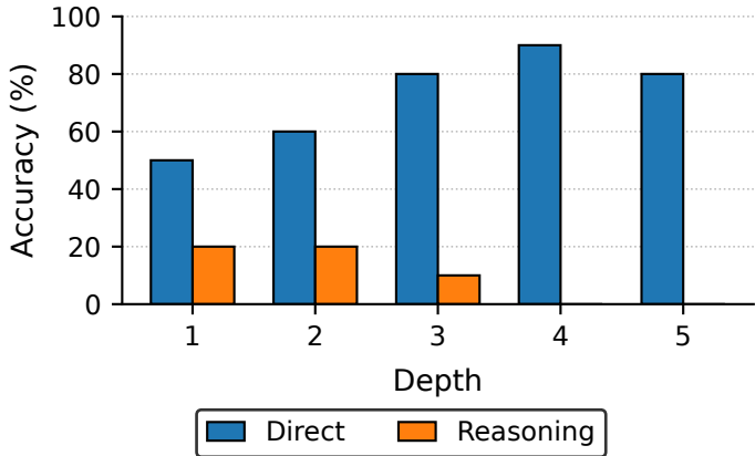
Accuracy vs Depth — GPT-5 (ProofWriter)
