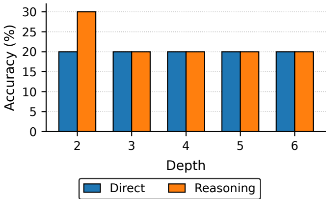
Accuracy vs Depth — LLaMA-3.1-8B (CLUTRR)
