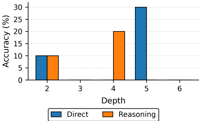
Accuracy vs Depth — Qwen-2.5-7B (CLUTRR)
