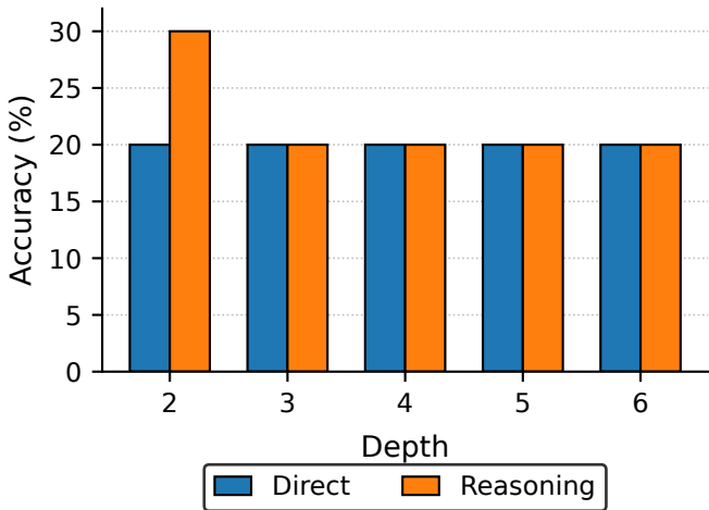
Accuracy vs Depth — LLaMA-3.1-8B (CLUTRR)
