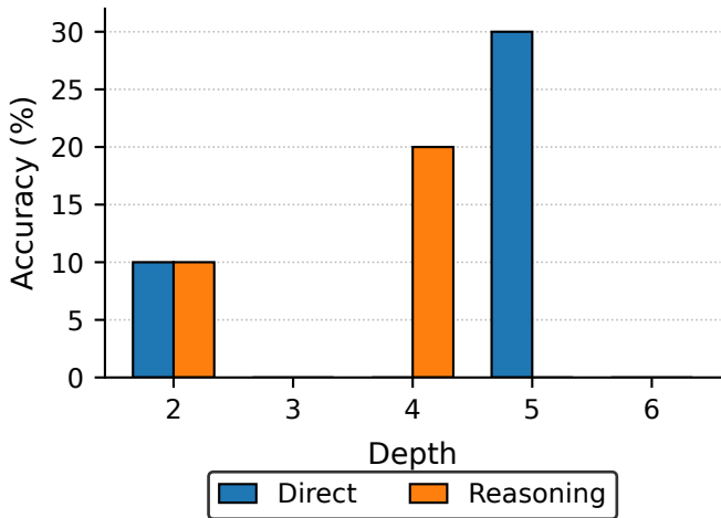
Accuracy vs Depth — Qwen-2.5-7B (CLUTRR)
