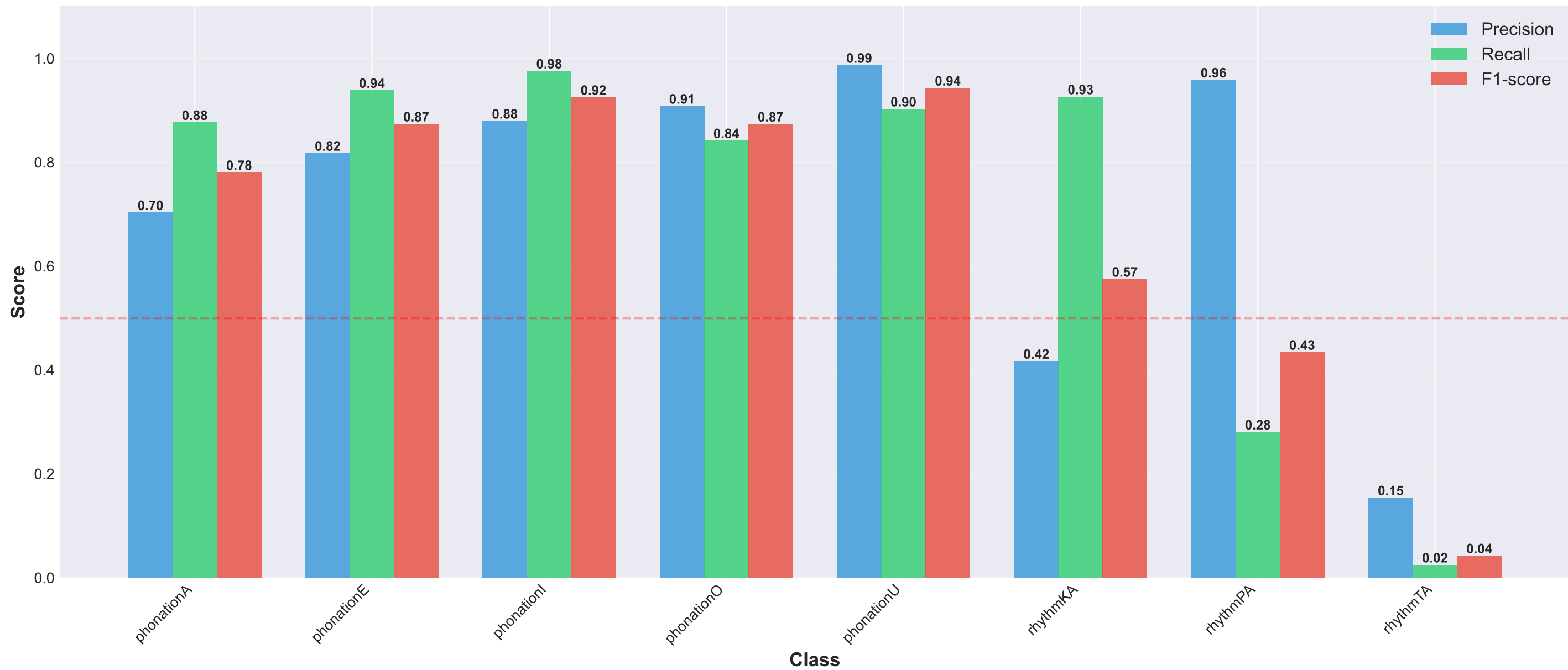
Per-Class Performance Metrics - Improved Model
