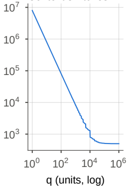
Context switches
