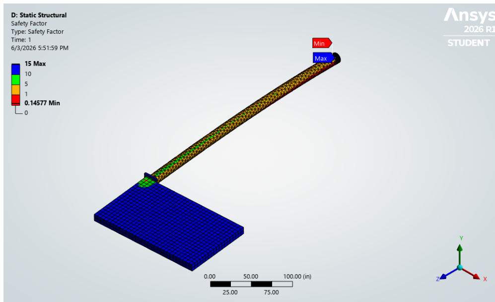
Figure 23: Factor of safety against tensile stress failure under impact load.
