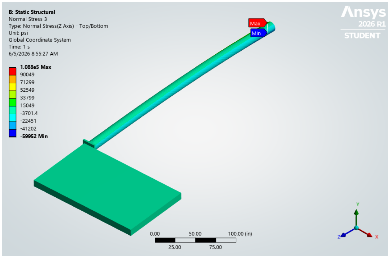
Figure 5: Normal stress distribution at Z-direction in the structure.
