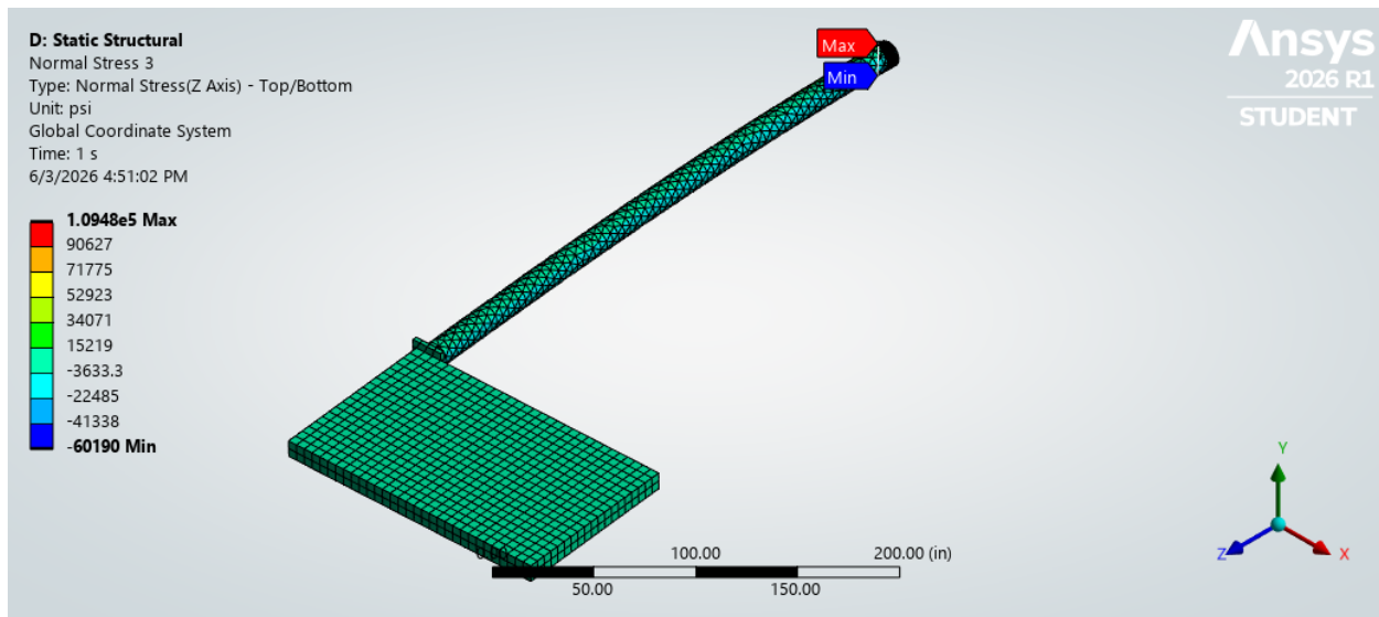
Figure 13: Normal stress distribution at Z-direction with galvanized steel material.
