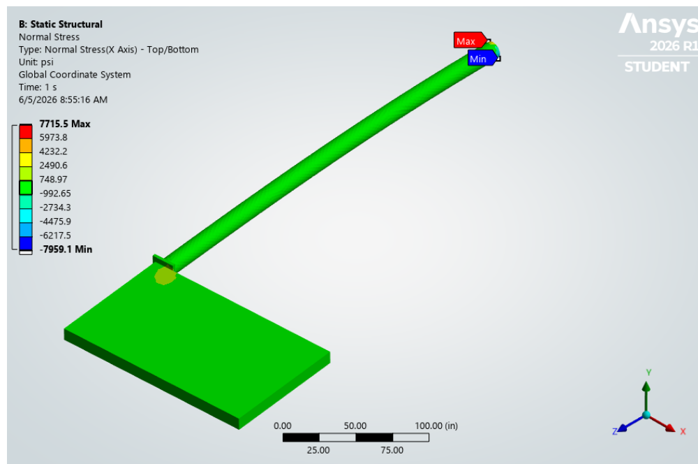
Figure 3: Normal stress distribution at X-direction in the structure.
