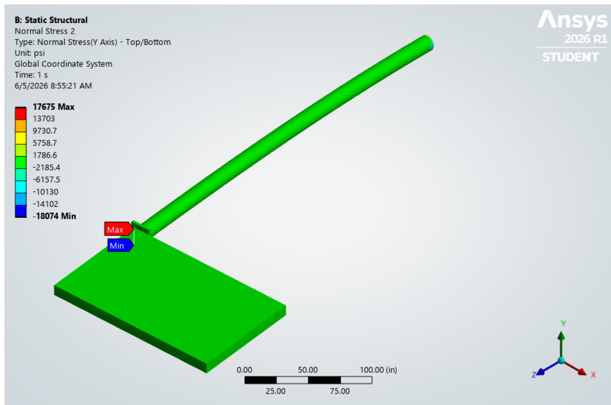
Figure 4: Normal stress distribution at Y-direction in the structure.
