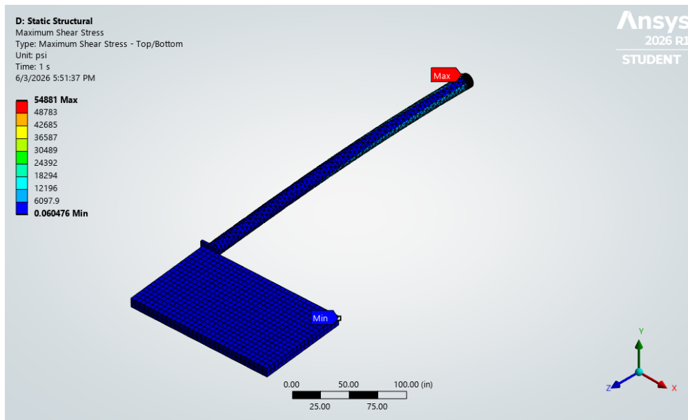
Figure 21: Maximum shear stress distribution under impact load.
