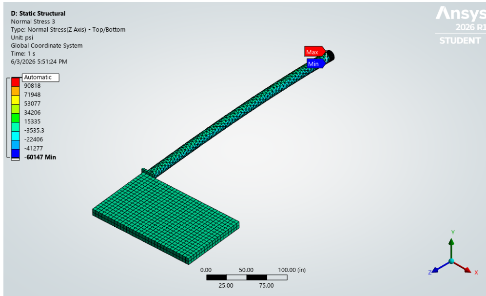
Figure 20: Normal stress distribution at Z-direction under impact load.
