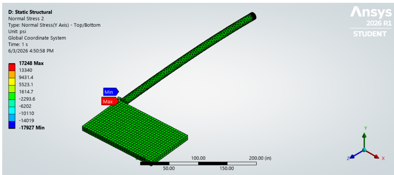
Figure 12: Normal stress distribution at Y-direction with galvanized steel material.
