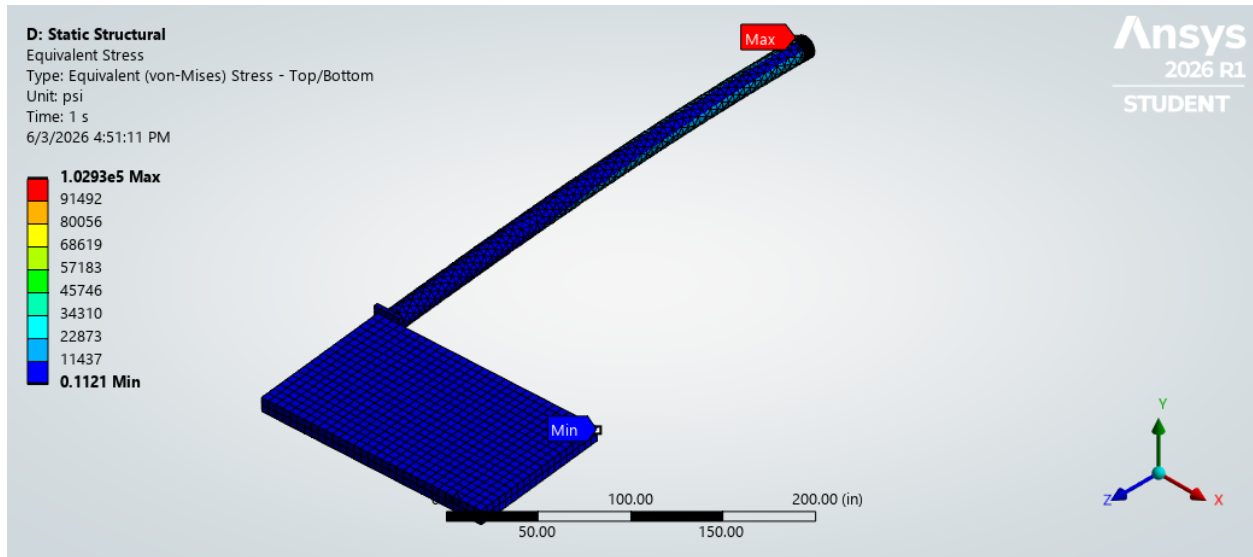
Figure 15: Equivalent stress distribution with galvanized steel material.
