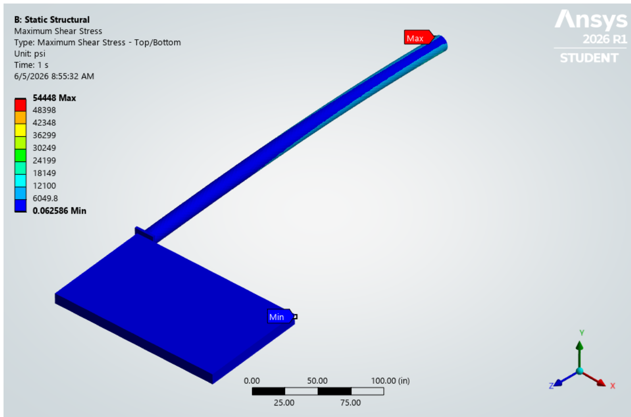
Figure 6: Maximum shear stress distribution in the structure.
