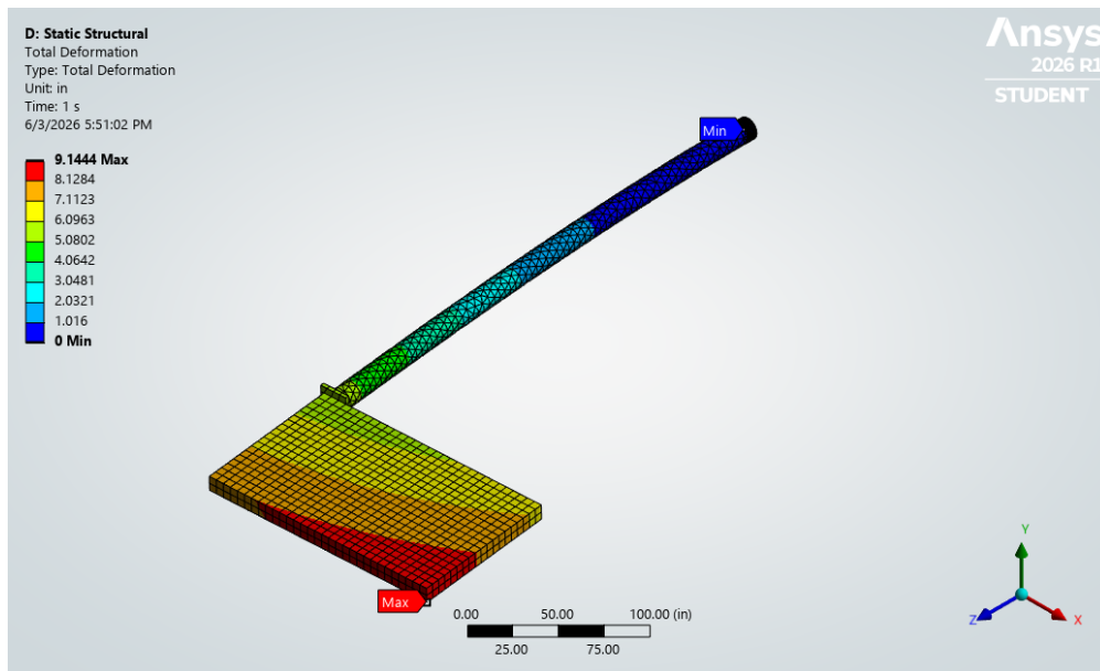
Figure 19: Total deformation of the structure under impact load.
