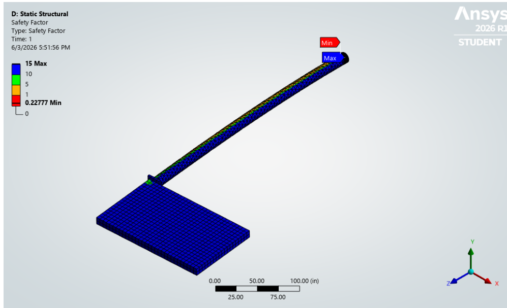
Figure 22: Factor of safety against shear failure under impact load.
