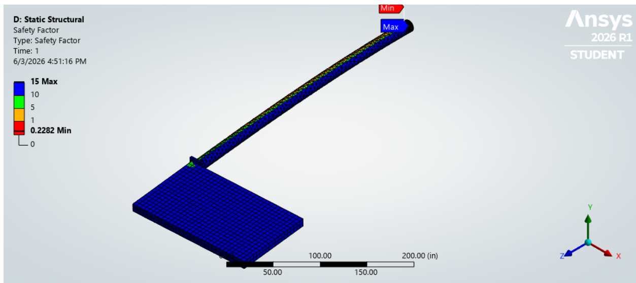
Figure 16: Factor of safety against shear failure with galvanized steel material.
