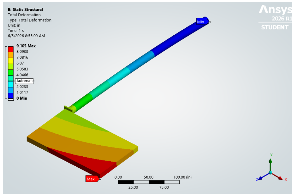
Figure 2: Total deformation of the structure under the applied loads.
