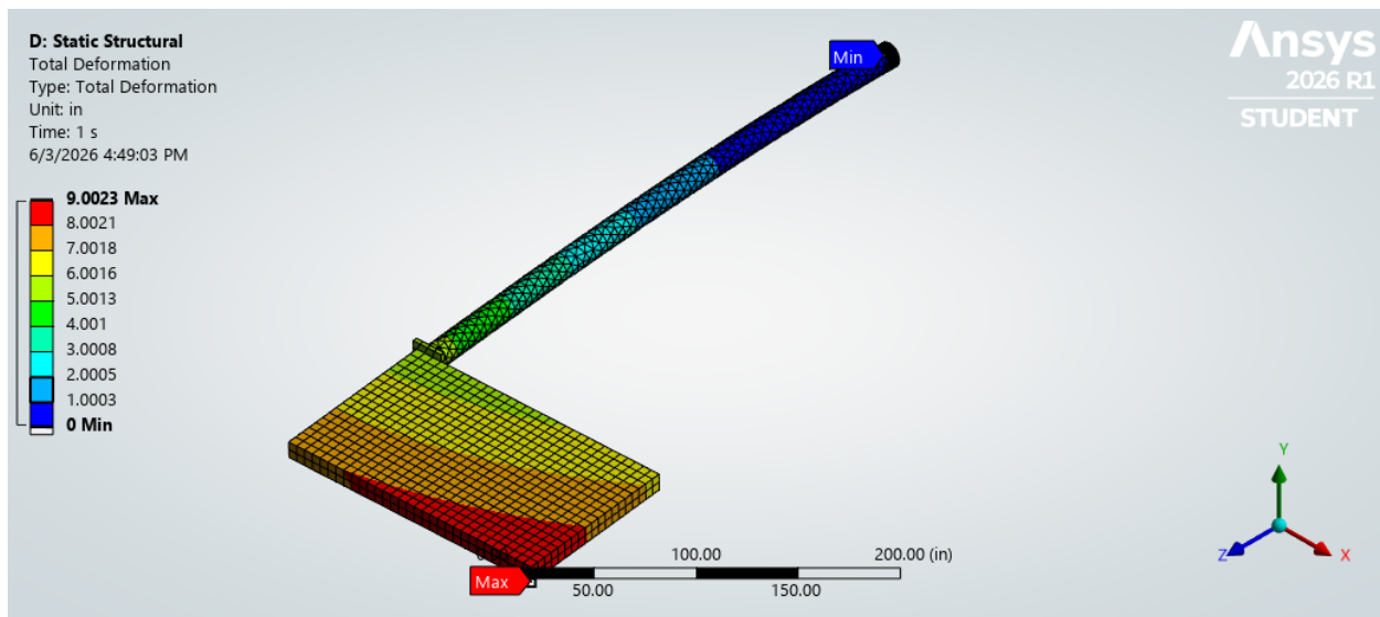
Figure 10: Total deformation of the structure with galvanized steel material.
