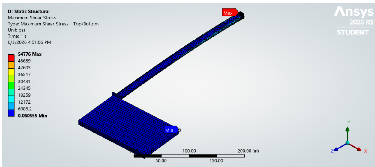
Figure 14: Maximum shear stress distribution with galvanized steel material.
