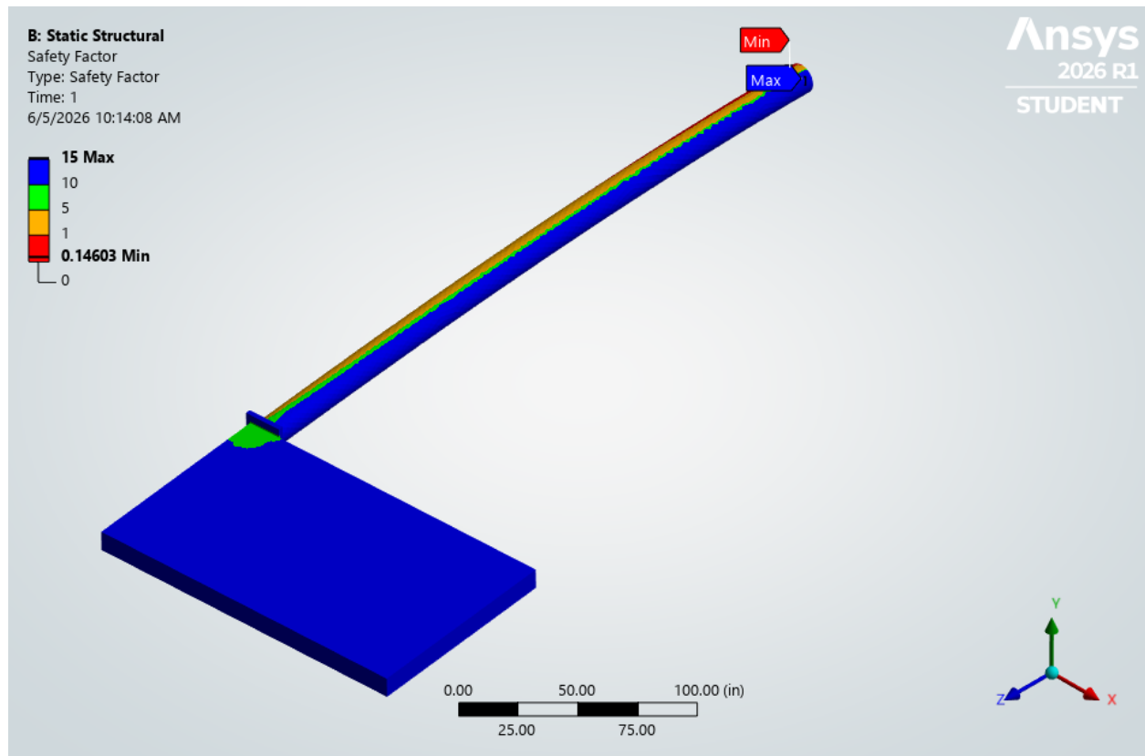
Figure 8: Factor of safety against shear failure.
