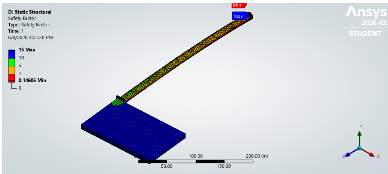
Figure 17: Factor of safety against tensile stress failure with galvanized steel material.
