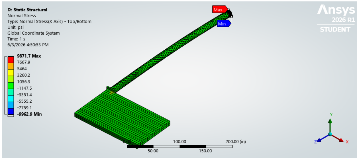
Figure 11: Normal stress distribution at X-direction with galvanized steel material.
