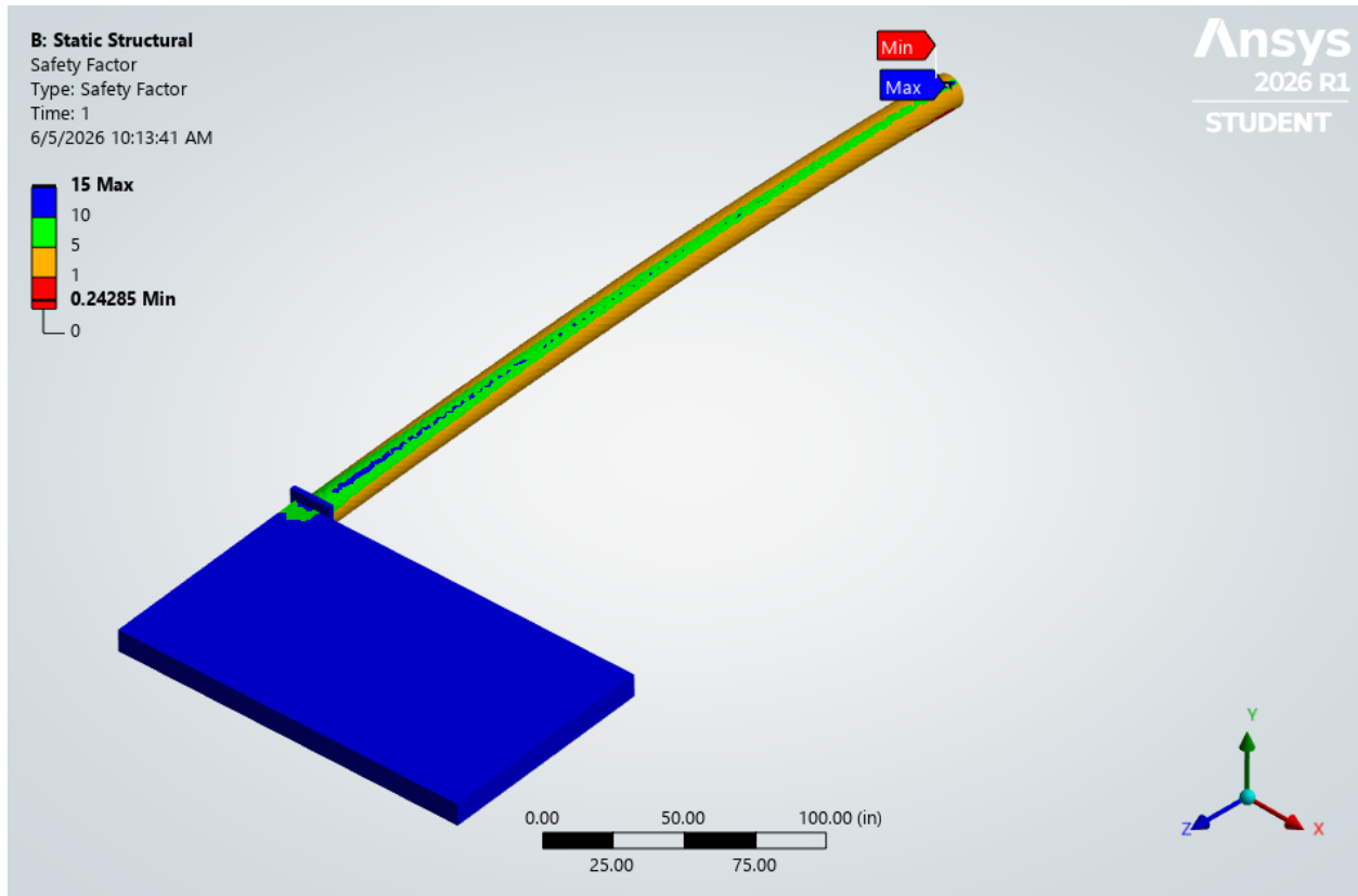
Figure 9: Factor of safety against tensile stress failure.
