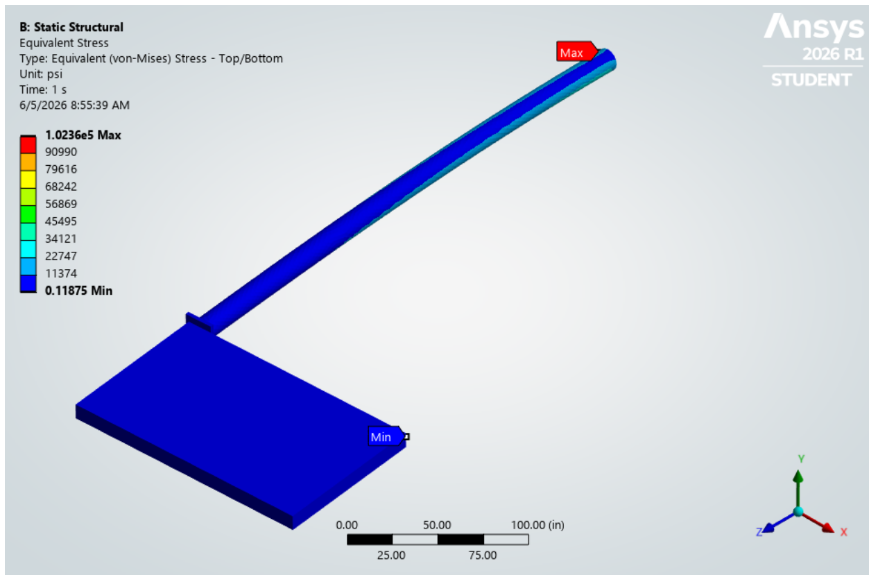
Figure 7: Equivalent stress distribution in the structure.
