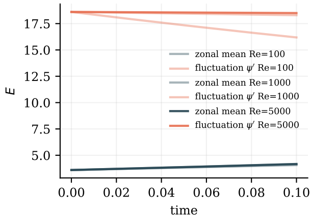
KE split: fluctuation \psi' (the reported statistic) zonal mean, which carries no method difference
