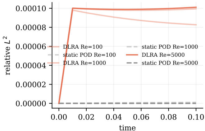
Trajectory divergence over the suite window, window t \leq 0.1 only; the crossover is bracketed in t \in [0.05, 0.2]
