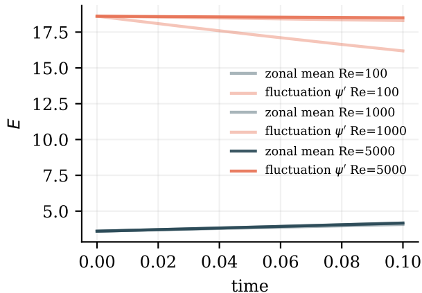
KE split: fluctuation \psi' (the reported statistic) and zonal mean, which carries no method difference
