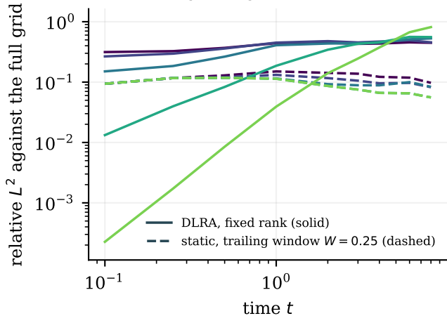
Error against horizon, by rank
