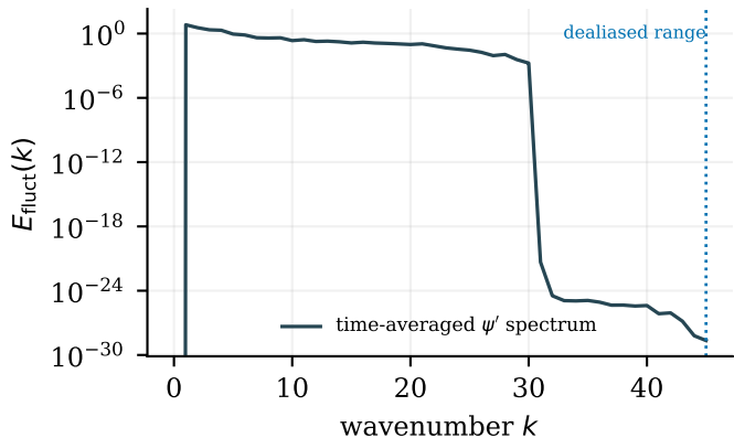
\psi' spectrum, t \in [4, 8] Z(k) omitted: enstrophy drifts, so it would average a moving quantity
