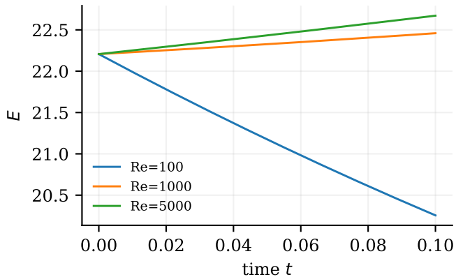
E(t) over the suite window
