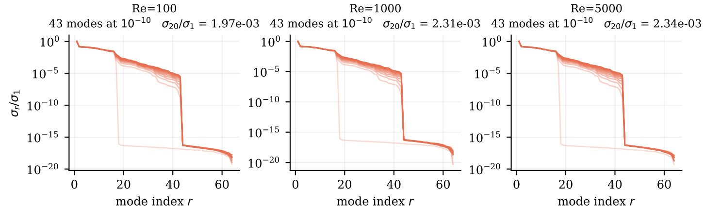
Singular-value decay of \psi at increasing times (darker = later)
