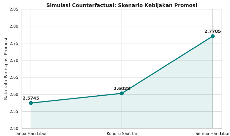
Gambar 6 Simulasi Counter-factual
