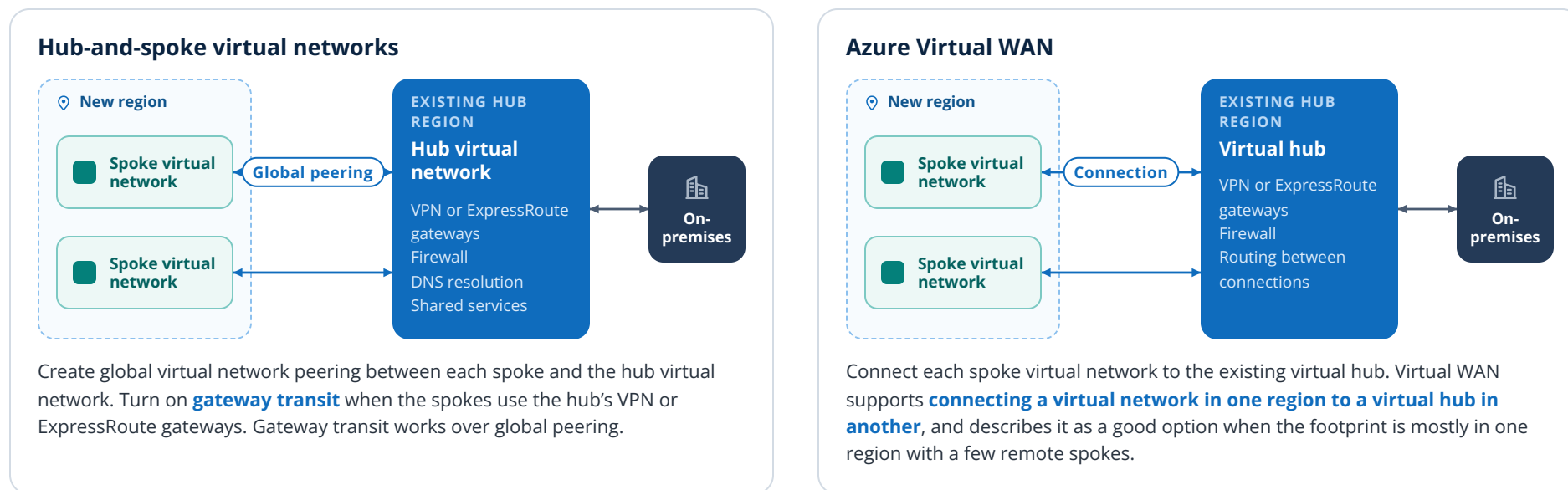
FIGURE 22 Two ways to reach the hub you already run. Spokes in the new region use the gateways, firewall, and shared services of a hub in another region. No hub is built in the new region.
