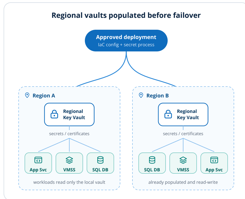
FIGURE 26 Pre-provisioned regional vaults. Applies to secrets and certificates. Design customer-managed keys (for example, SQL TDE) separately; see the customer-managed keys scenario on the next page.
