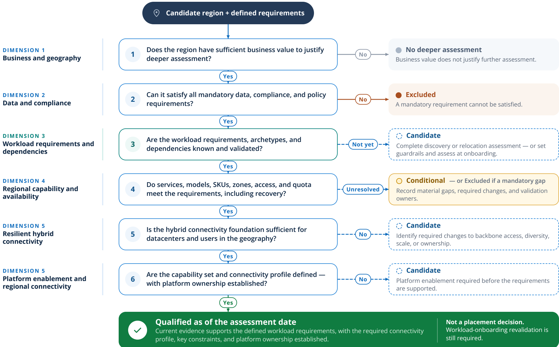
FIGURE 15 Regional qualification decision tree. Filters first, then technical fit, then platform readiness. Candidate and conditional options return to the tree when validation or enablement is complete, or conditions change.
