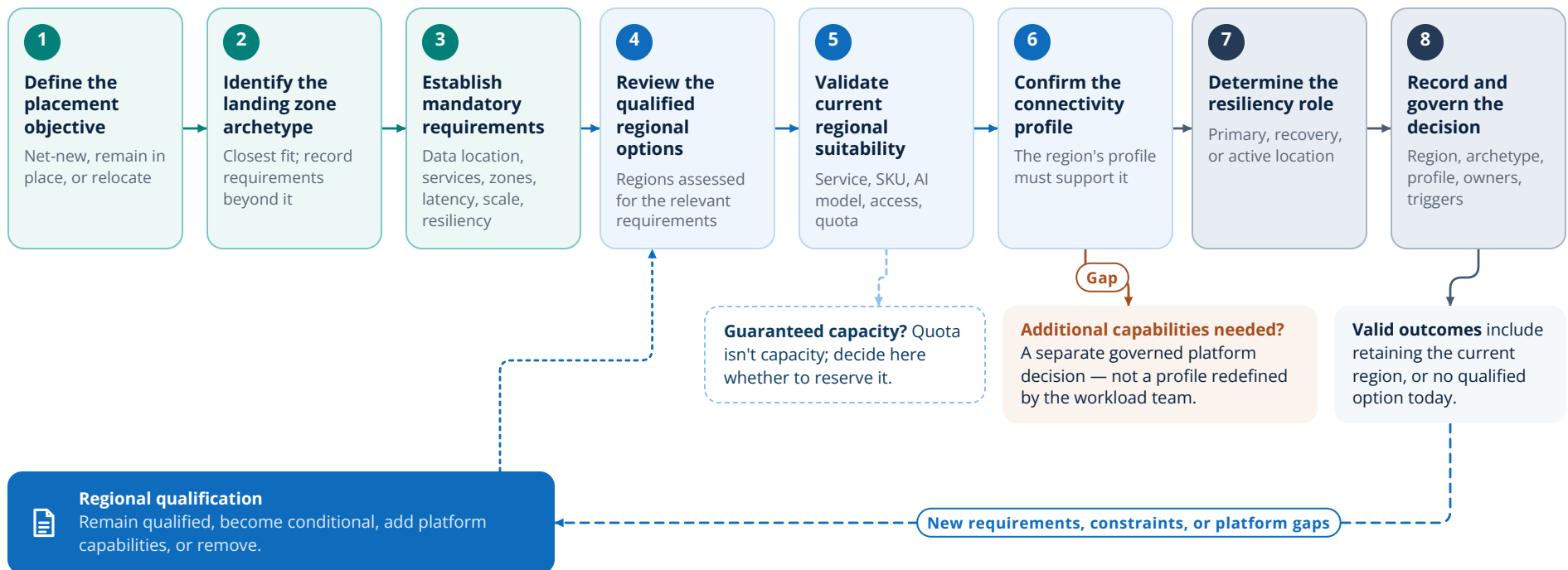
FIGURE 23 Workload placement using qualified options. Teal steps describe the workload, blue steps match it to regional options, and slate steps decide and govern. Onboarding findings return to regional qualification, closing the loop between platform readiness and workload adoption.
