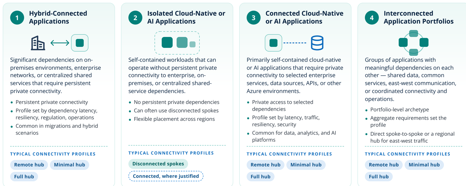
FIGURE 16 Four Workload Landing Zone archetypes. Grouped by the platform connectivity and dependency capabilities each requires. Profile relationships are detailed in Figure 17.
