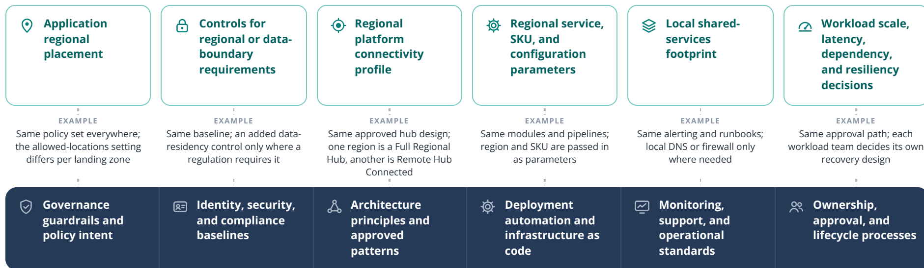
FIGURE 25 What stays consistent and what adapts. Placement varies, governance does not; profiles vary, approved patterns do not.
