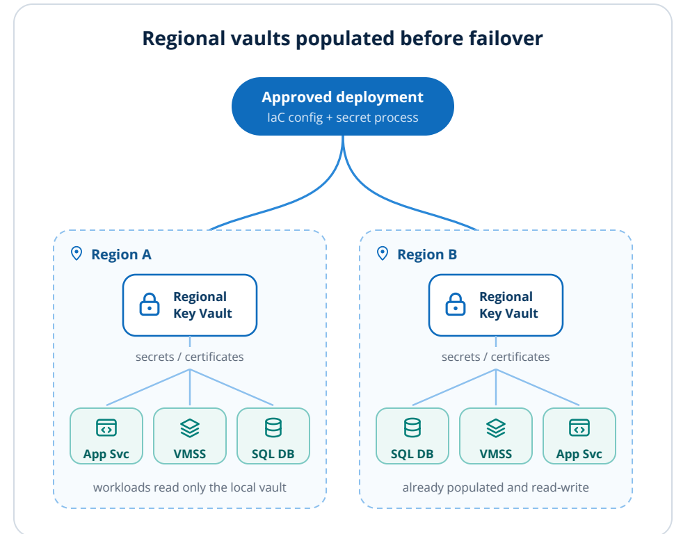
FIGURE 27 Pre-provisioned regional vaults. Applies to secrets and certificates. Design customer-managed keys (for example, SQL TDE) separately; see the customer-managed keys scenario on the next page.
