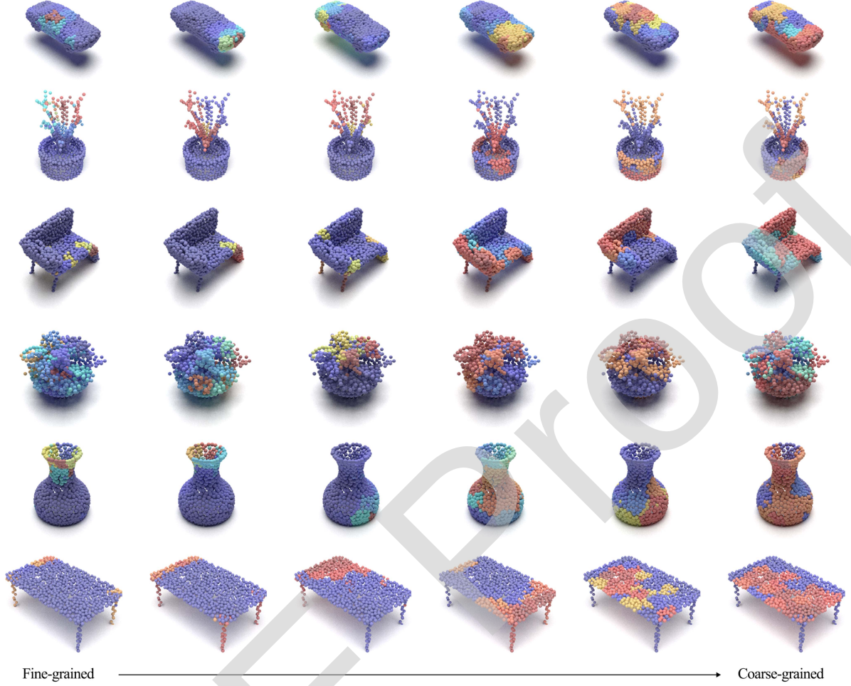
Fig. 6. Visualization of attention distributions induced by our fused multi-granular geometric prompts. Samples are obtained on the ModelNet40 dataset. Warm colors correspond to higher attention scores.
