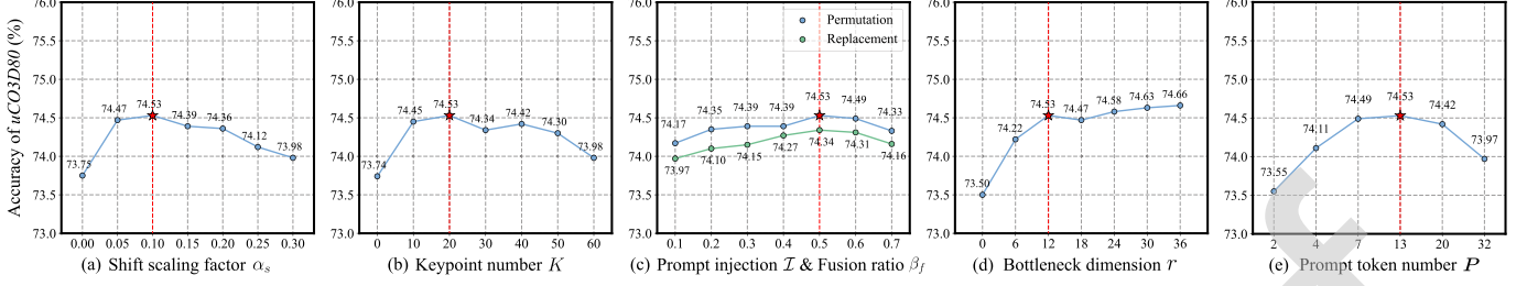
Fig. 7. Ablation results on hyperparameter settings. The settings highlighted by red dashed lines denote those used in our proposed approach.
