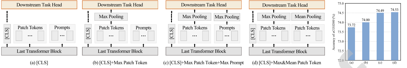
Fig. 9. Ablation study analyzing the impact of different feature inputs fed into the downstream head and their contribution to performance.
