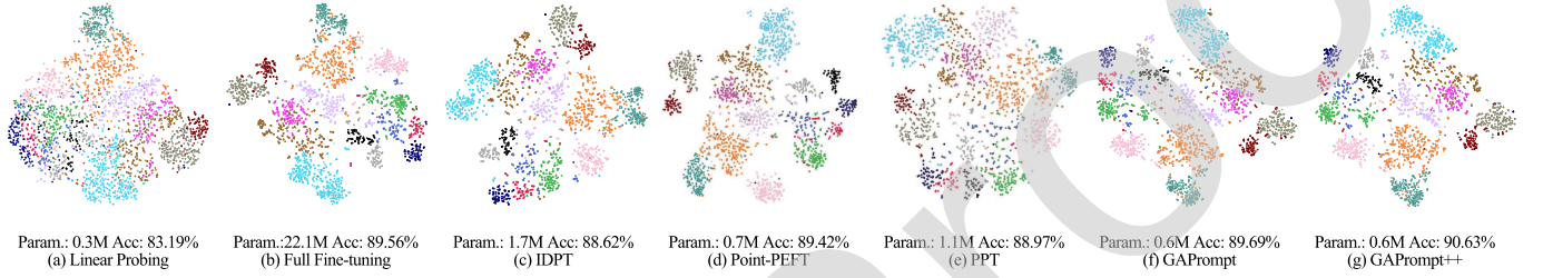
Fig. 8. The t-SNE visualizations of test features on the PB_T50_RS split of ScanObjectNN . The embeddings are obtained from the last block of a pre-trained Point-PQAE [39] under different parameter-efficient adaptation strategies.
