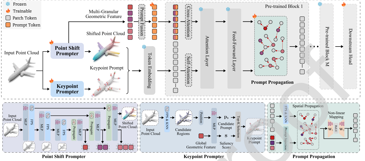
Fig. 5. The overall pipeline of GAPrompt++. Given an input point cloud, the Point Shift Prompter extracts multi-granular geometric features and performs fine-grained point shifts, while the Keypoint Prompter identifies salient local structures and generates instance-specific keypoint prompts. During feature extraction, learnable prompt tokens are prepended and fused with multi-granular geometric features and then are processed by the Prompt Propagation, which injects geometric cues across the model hierarchy. Finally, the propagated tokens are passed through the pre-trained backbone to make downstream predictions.
