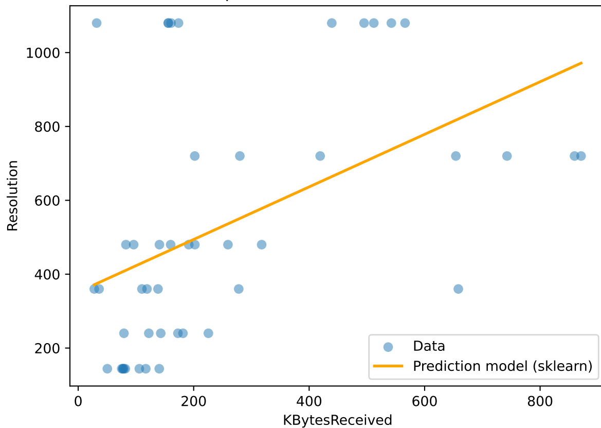
Data and prediction of OLS model (scikit-learn)
