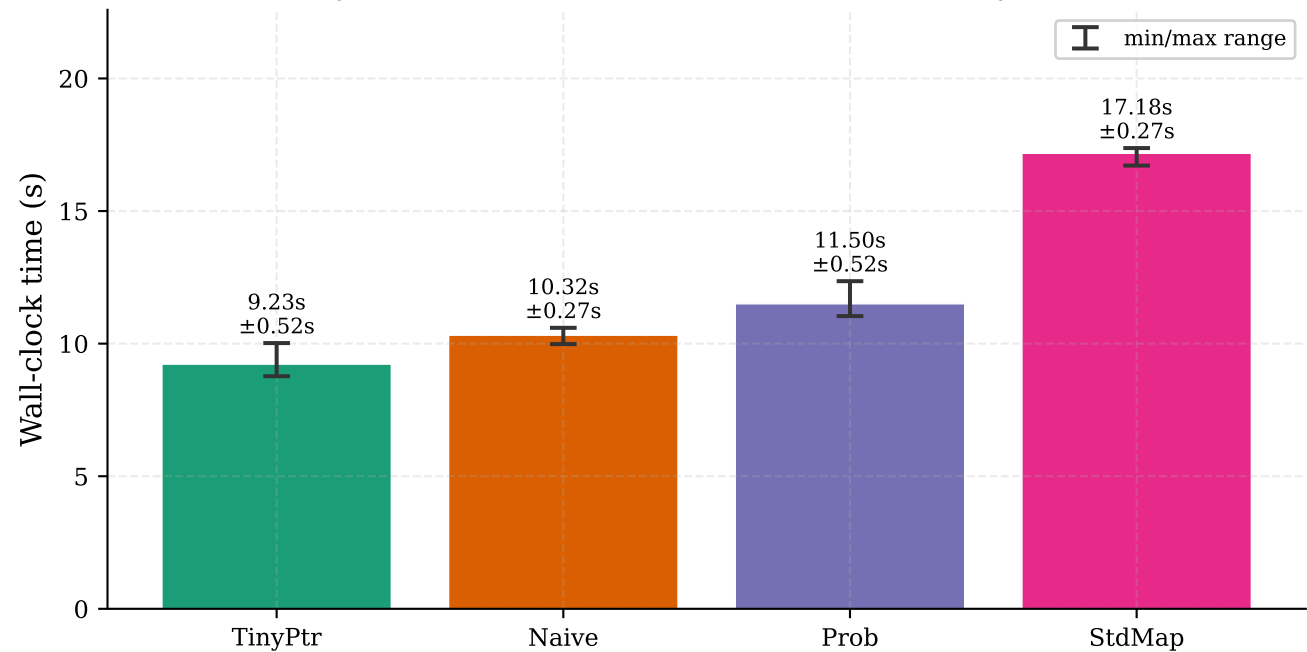
Figure 7: End-to-End Crack Time (hyperfine, 5 runs, 2 warmups, 4 threads, entry \sim 7\text{M} )
