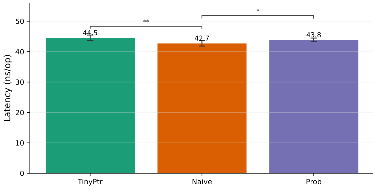
Custom Implementations (zoomed, 95% CI)
