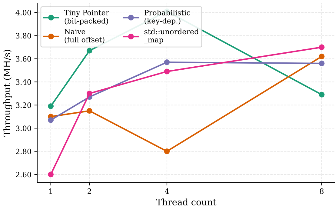
Figure 3: Cracker Throughput Scaling (full RockYou, mid-list target)
