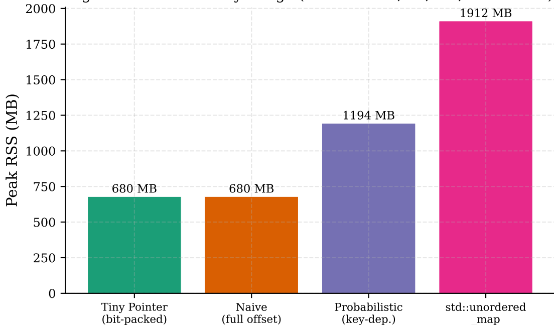
Figure 5: Peak Memory Usage (full RockYou, 14,344,391 entries)
