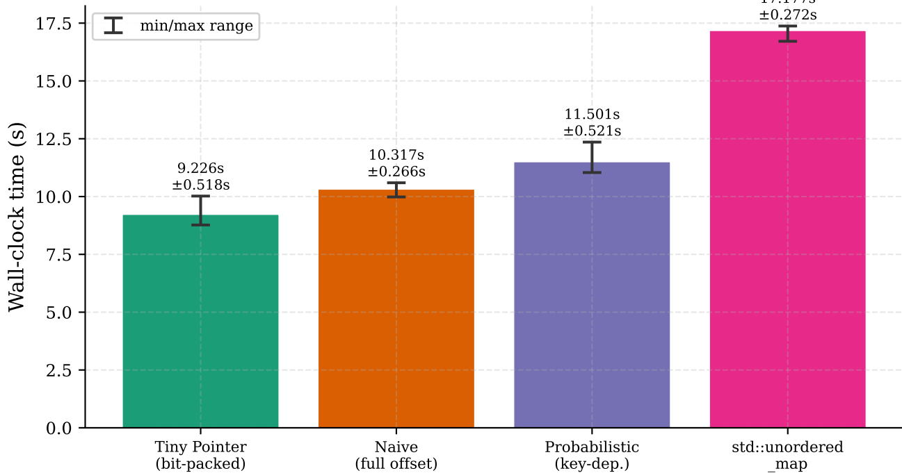
Figure 7: End-to-End Crack Time (hyperfine, 5 runs, 2 warmups, 4 threads)
