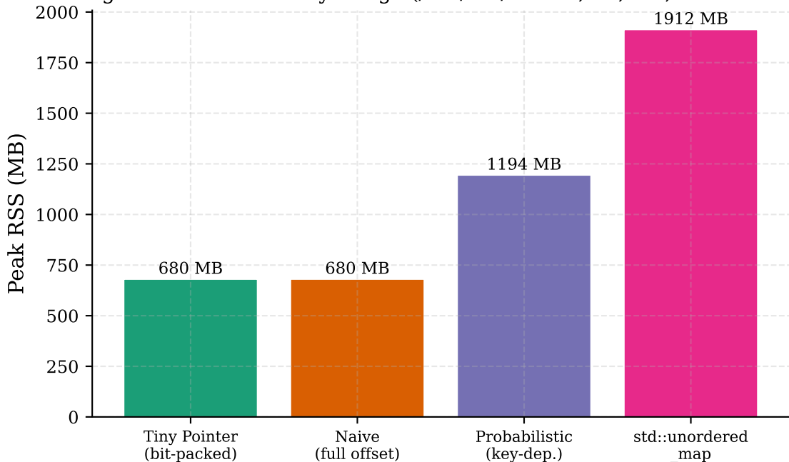
Figure 8: Peak Memory Usage (/usr/bin/time -v, 14,344,391 entries)
