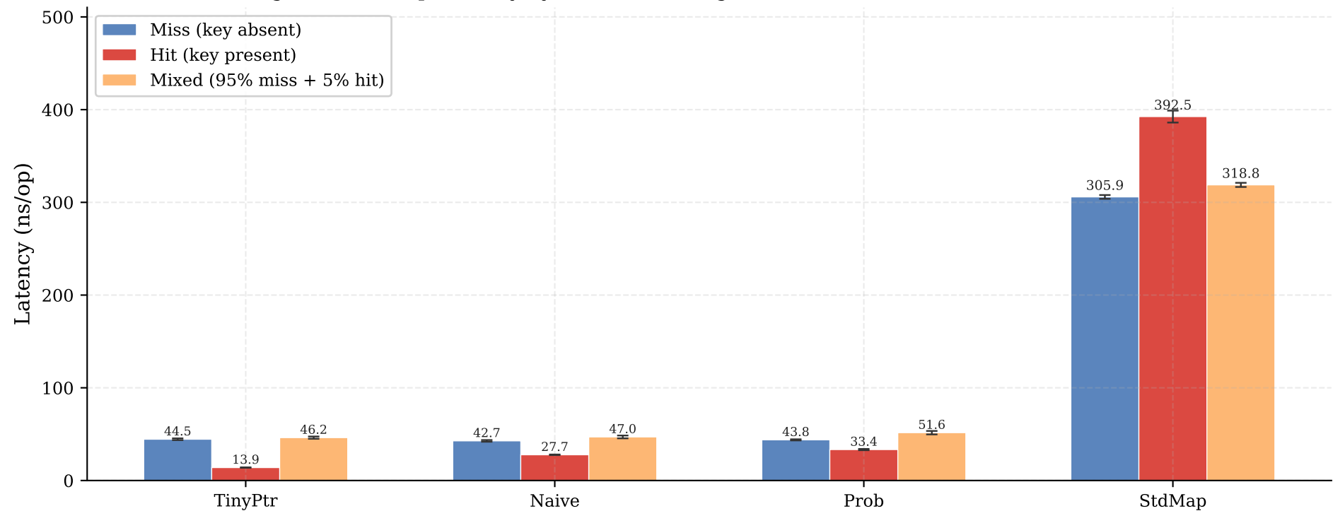
Figure 2: Lookup Latency by Workload (Google Benchmark, n=5, error bars = 95% CI)
