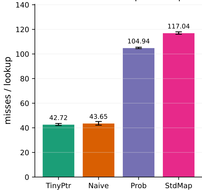
LLC Cache Misses per Lookup
