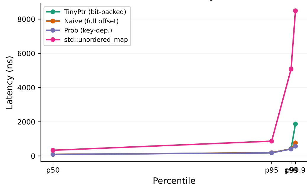
Full Percentile Range
