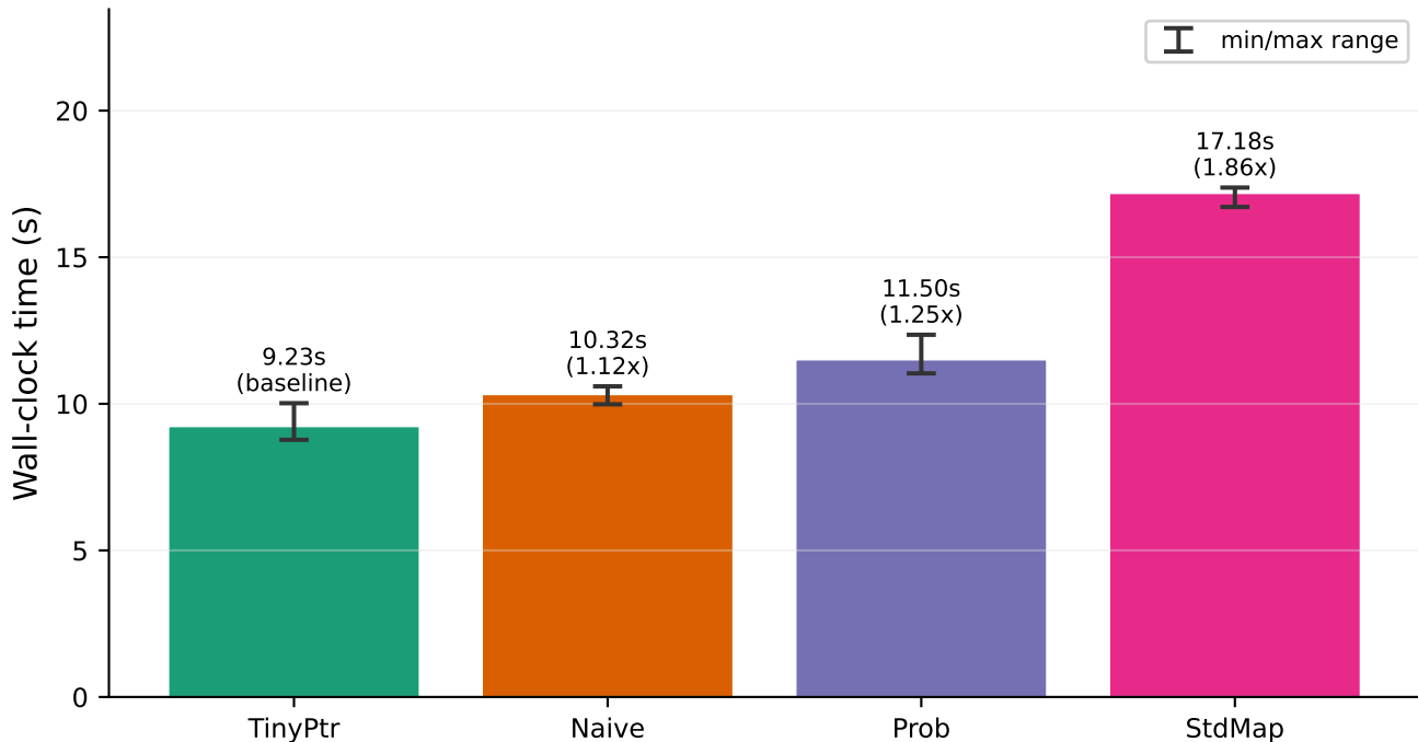
End-to-end crack time (hyperfine, 5 runs, 2 warmups, 4 threads)
