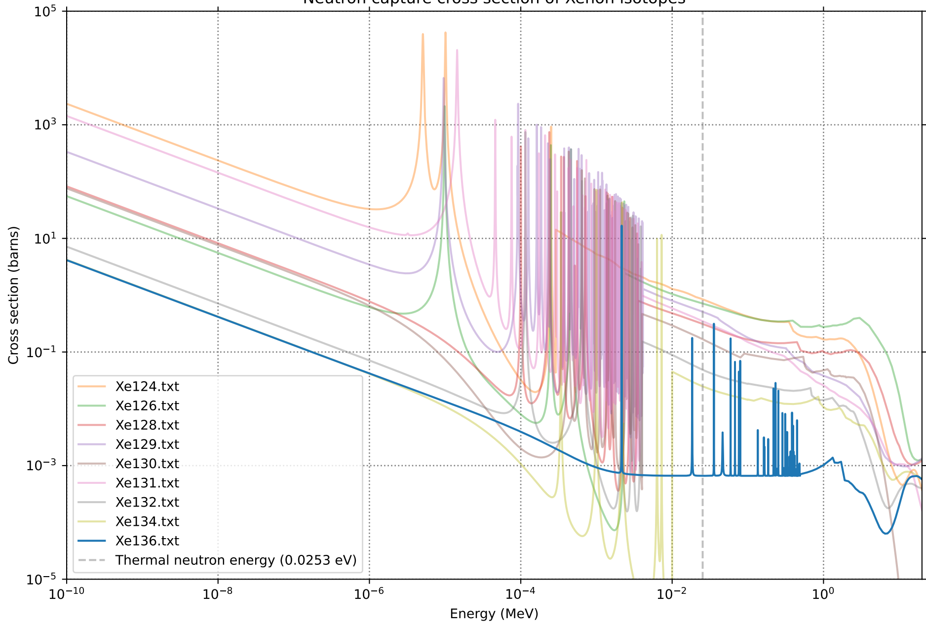
Neutron capture cross section of Xenon isotopes
