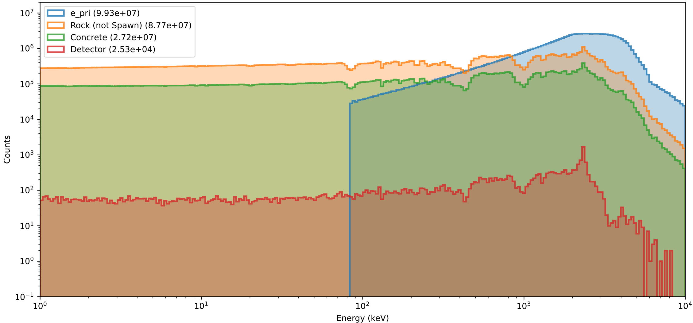
Energy distribution entering different volumes (Rock EnergyDist)
