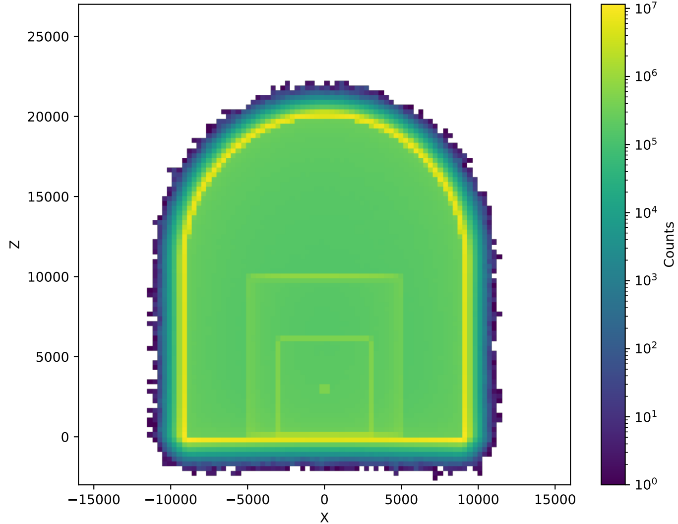
NeutronActivations (10cm, NoAbsorber, 2.44e+09)
