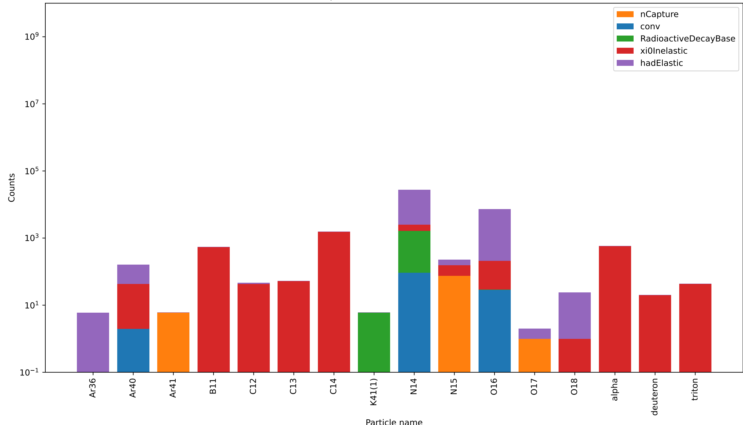
Neutron activation products in the Absorber (10cm NoAbsorber)
